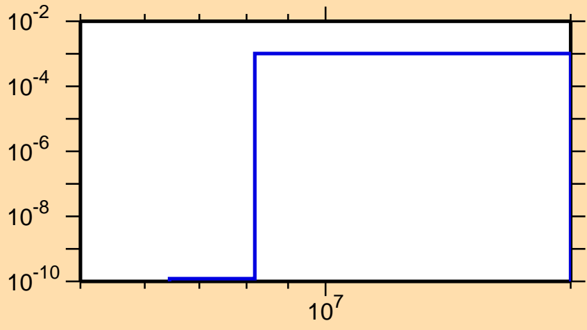
\sigma vs. E for ^{180}\text{Ta}(n,d)
