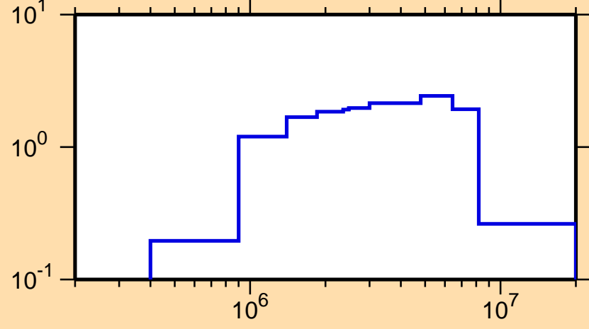
\sigma vs. E for ^{180}\text{Ta}(n,n\text{cont.})
