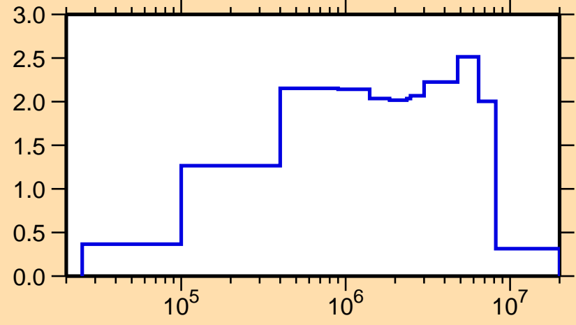
\sigma vs. E for ^{180}\text{Ta}(n,\text{inel.})
