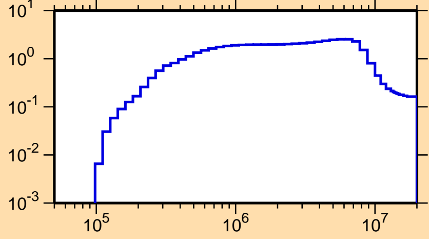
\sigma vs. E for ^{180}\text{Ta}(n,\text{inel.})
