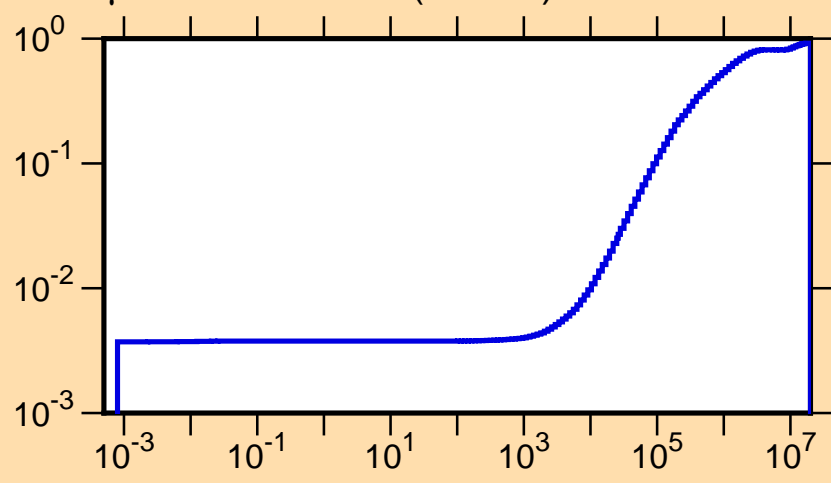
\mu vs. E for ^{181}\text{Ta}(\text{mt251})
