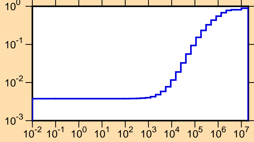
\mu vs. E for ^{181}\text{Ta}(\text{mt251})
