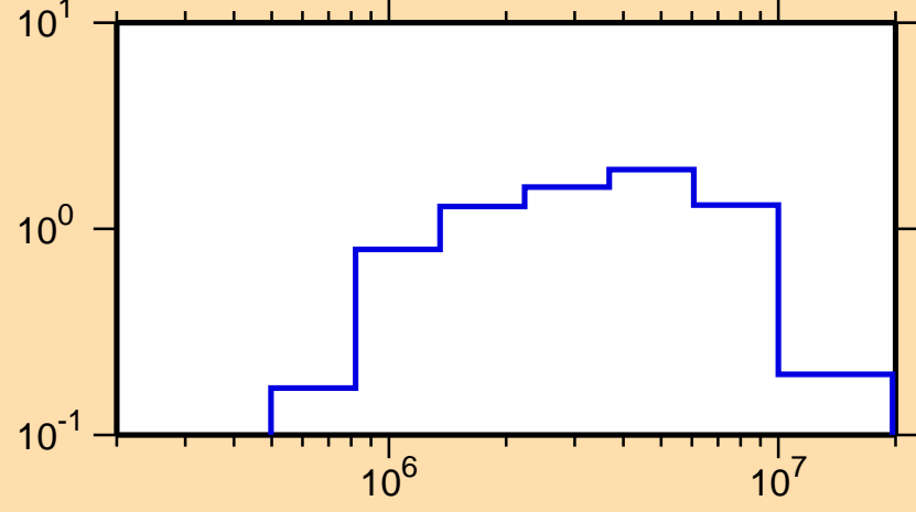
\sigma vs. E for ^{182}\text{Ta}(n,n\text{cont.})
