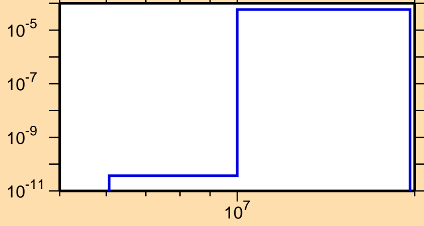
\sigma vs. E for ^{182}\text{Ta}(n,t)
