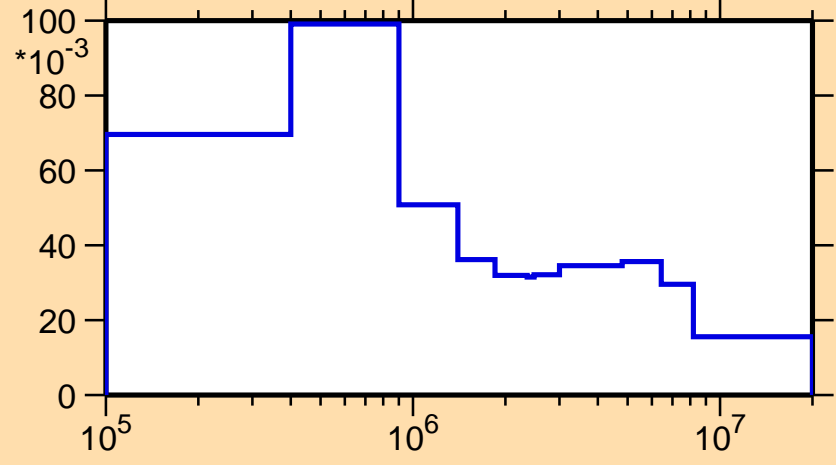
\sigma vs. E for ^{182}\text{Ta}(n,n_4)
