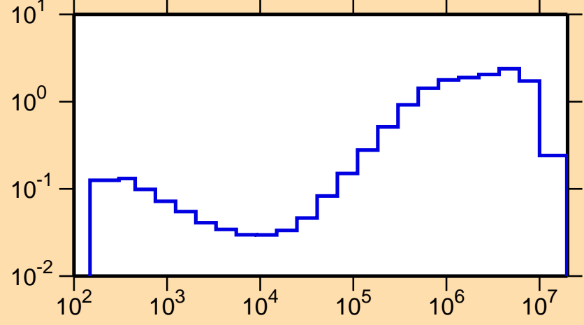
\sigma vs. E for ^{182}\text{Ta}(n,\text{inel.})
