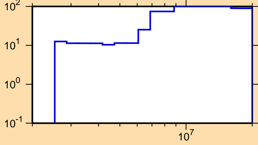
\Delta\sigma/\sigma vs. E for ^{184}\text{Ta}(n,n\text{cont.})
