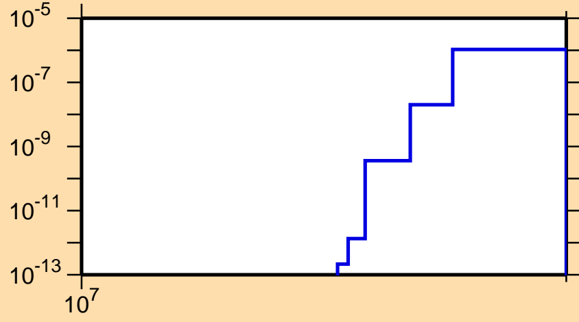
\sigma vs. E for ^{184}\text{Ta}(n,2np)
