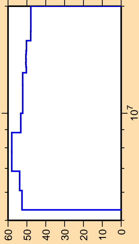
\Delta\sigma/\sigma vs. E for ^{184}\text{Ta}(n,n_1)
