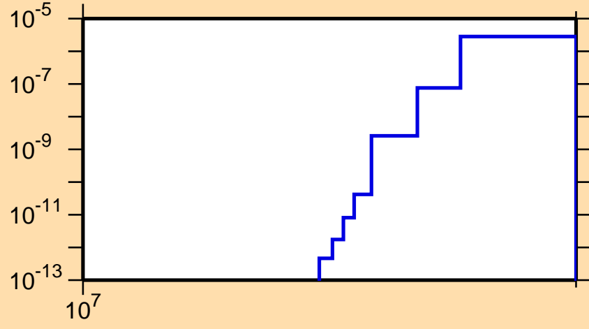
\sigma vs. E for ^{184}\text{Ta}(n,nt)
