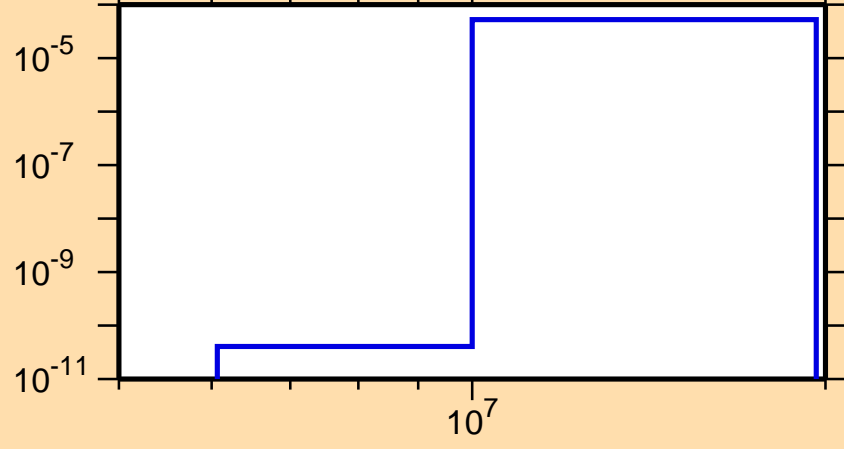
\sigma vs. E for ^{184}\text{Ta}(n,t)
