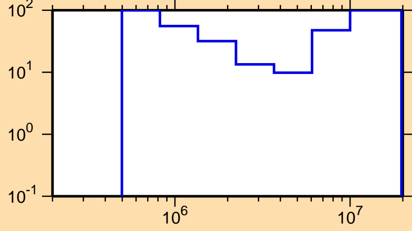
\Delta\sigma/\sigma vs. E for ^{184}\text{Ta}(n,n\text{cont.})
