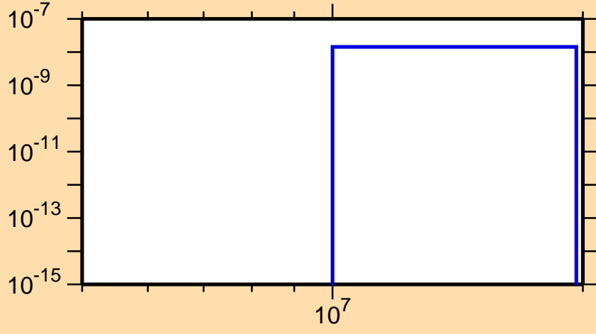
\sigma vs. E for ^{184}\text{Ta}(n,2n\alpha)
