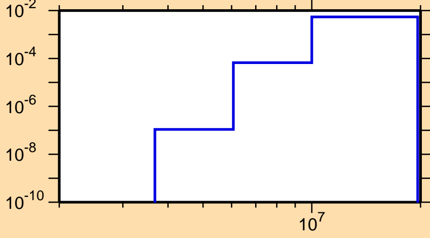
\sigma vs. E for ^{184}\text{Ta}(n,p)
