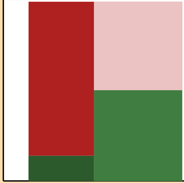
\Delta\sigma/\sigma vs. E for ^{185}\text{Ta}(n,2n)
