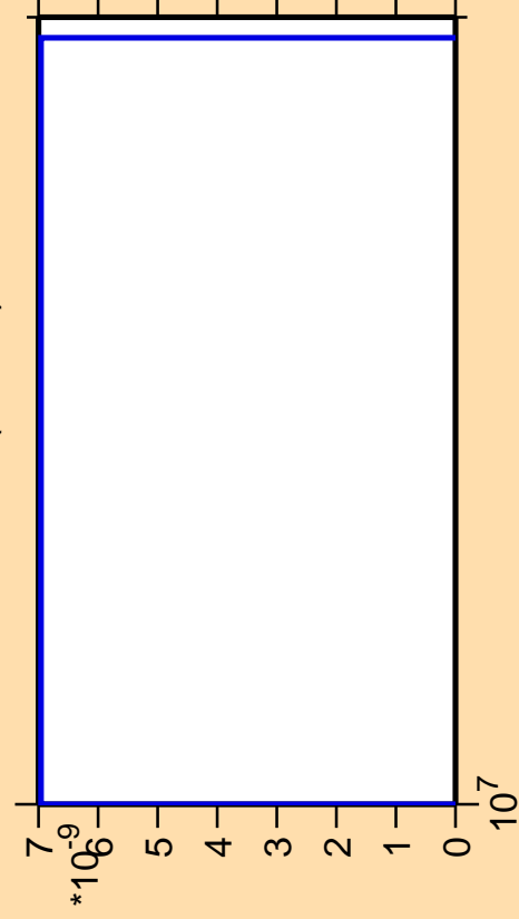
\Delta\sigma/\sigma vs. E for ^{185}\text{Ta} (mt 42)
