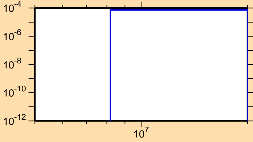
\sigma vs. E for ^{185}\text{Ta}(n,d)
