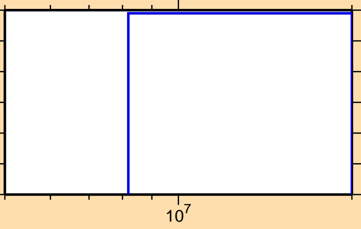
\sigma vs. E for ^{185}\text{Ta}(n,2n\alpha)
