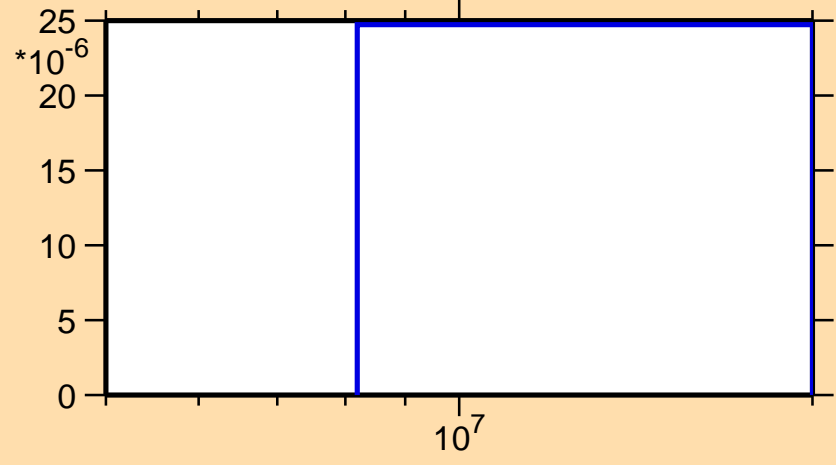
\sigma vs. E for ^{185}\text{Ta}(n,t)
