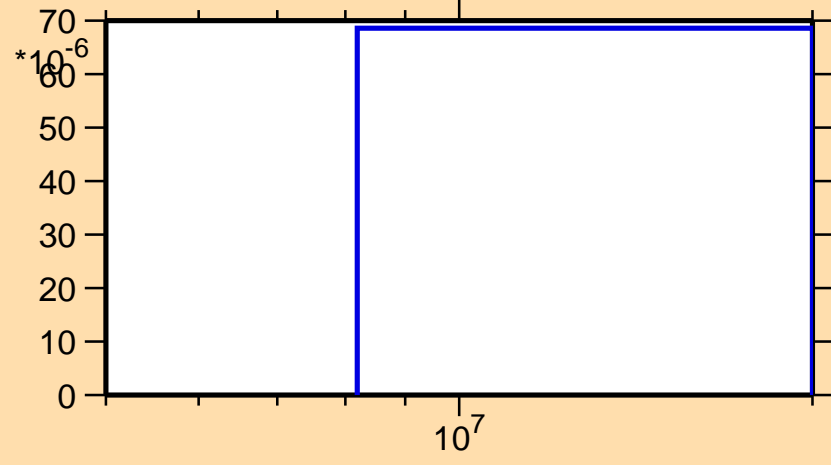
\sigma vs. E for ^{185}\text{Ta}(n,np)
