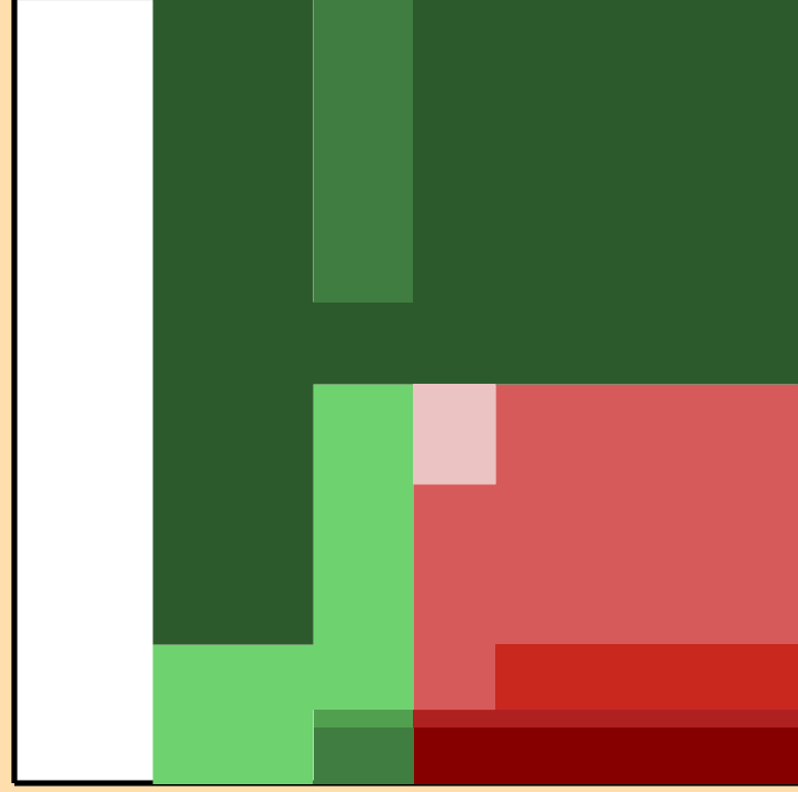
\Delta\sigma/\sigma vs. E for ^{185}\text{Ta}(n,p)
