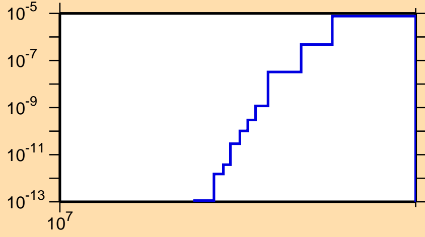
\sigma vs. E for ^{186}\text{Ta}(n,\text{nd})
