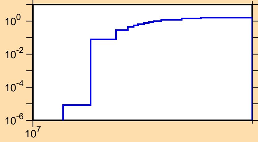
\sigma vs. E for ^{186}\text{Ta}(n,3n)
