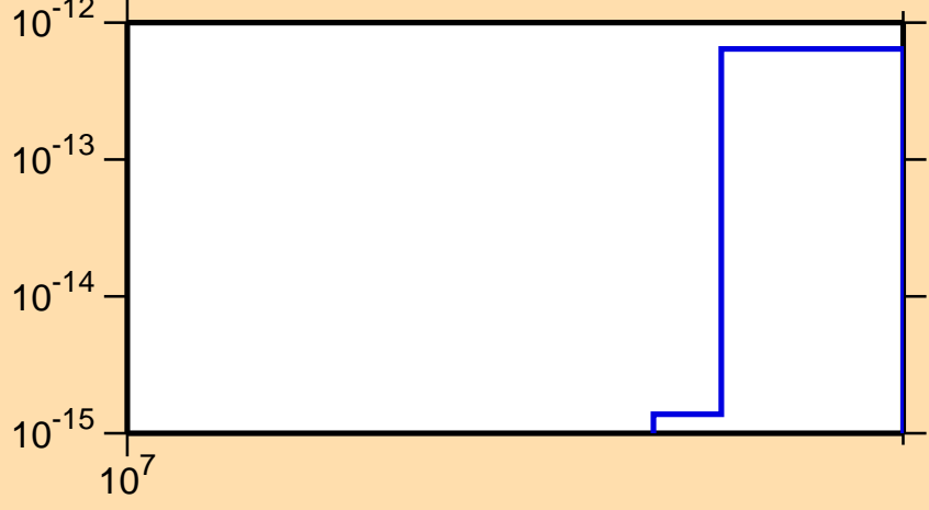
\sigma vs. E for ^{186}\text{Ta}(n,\text{He}3)
