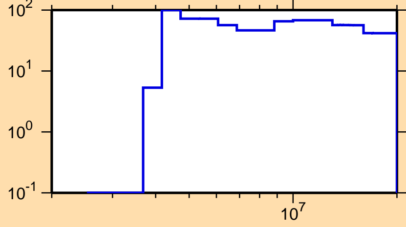
\Delta\sigma/\sigma vs. E for ^{186}\text{Ta}(n,p)
