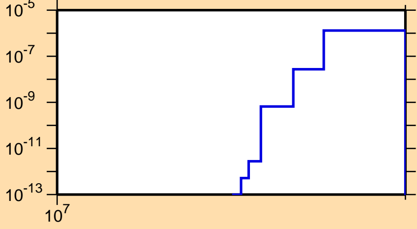
\sigma vs. E for ^{186}\text{Ta}(n,2np)
