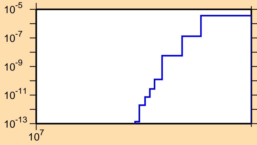
\sigma vs. E for ^{186}\text{Ta}(n,nt)
