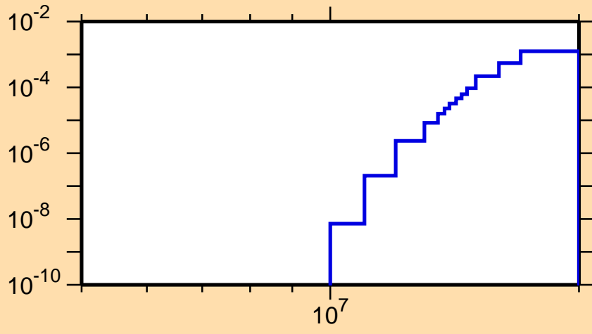
\sigma vs. E for ^{186}\text{Ta}(n,d)
