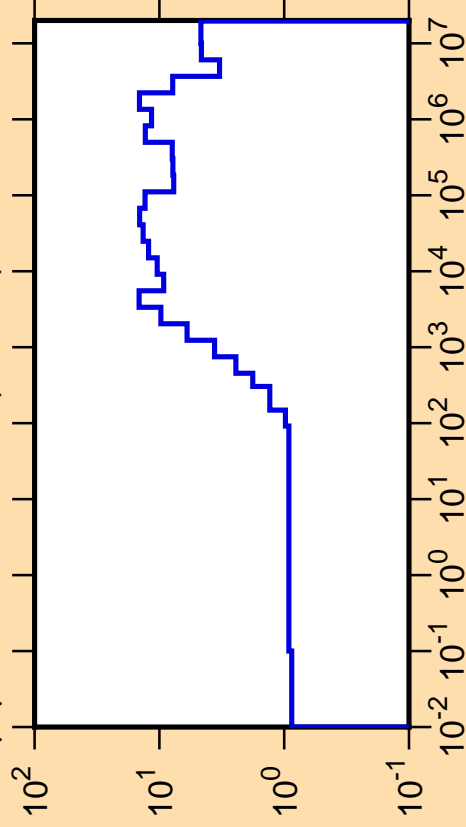
\Delta\mu/\mu vs. E for ^{186}\text{Ta}(\text{mt251})
