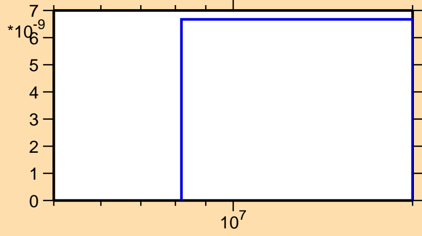
\sigma vs. E for ^{186}\text{Ta}(n,2n\alpha)
