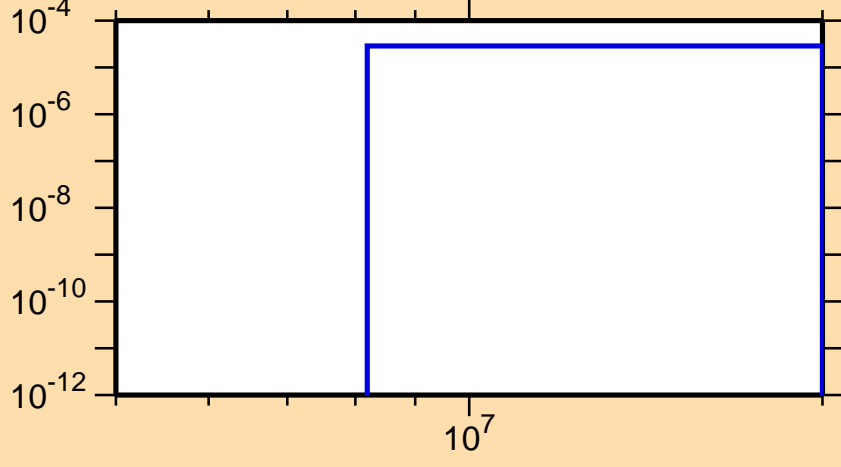
\sigma vs. E for ^{186}\text{Ta}(n,t)
