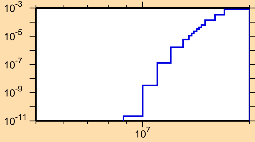
\sigma vs. E for ^{187}\text{Ta}(n,d)
