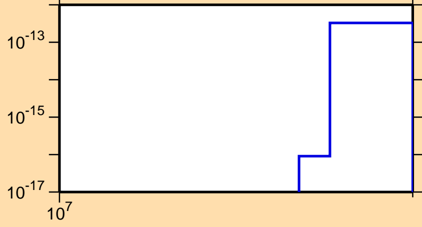
\sigma vs. E for ^{187}\text{Ta}(n,3n\alpha)
