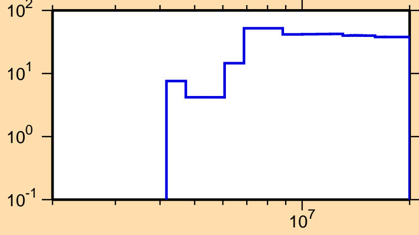
\Delta\sigma/\sigma vs. E for ^{187}\text{Ta}(n,n\text{cont.})
