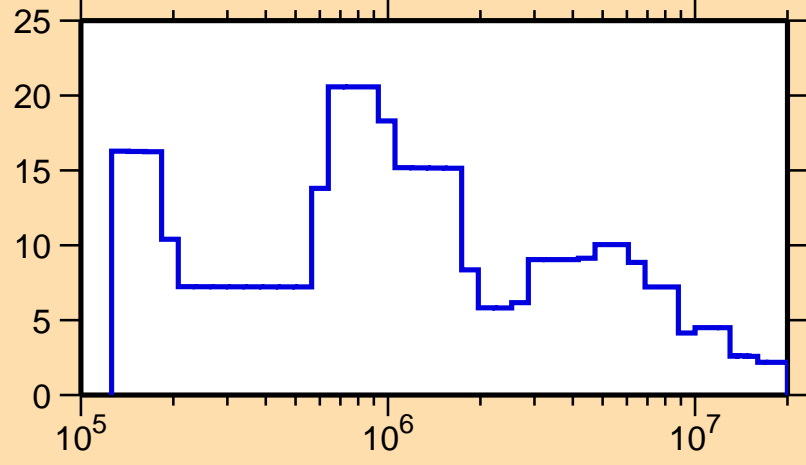
\Delta\sigma/\sigma vs. E for ^{187}\text{Ta}(n,tot.)
