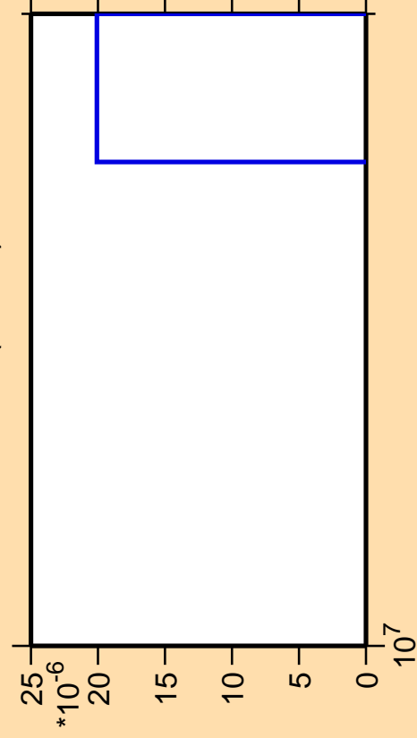
\Delta\sigma/\sigma vs. E for ^{187}\text{Ta} (mt 42)
