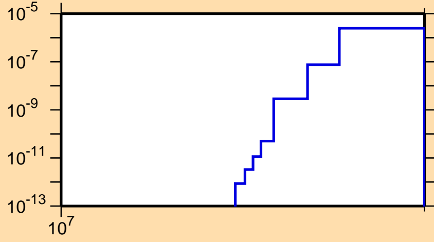
\sigma vs. E for ^{187}\text{Ta}(n,nt)
