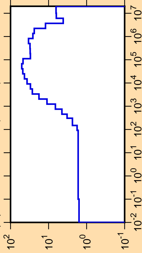
\Delta\mu/\mu vs. E for ^{187}\text{Ta}(\text{mt251})
