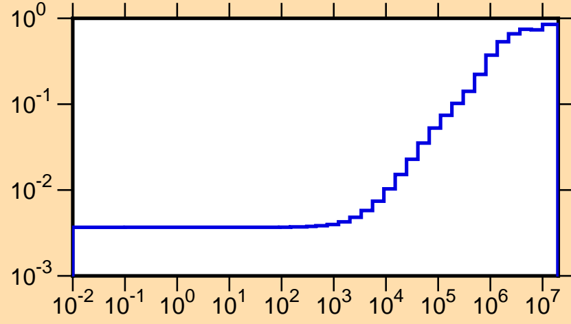
\mu vs. E for ^{187}\text{Ta}(\text{mt251})
