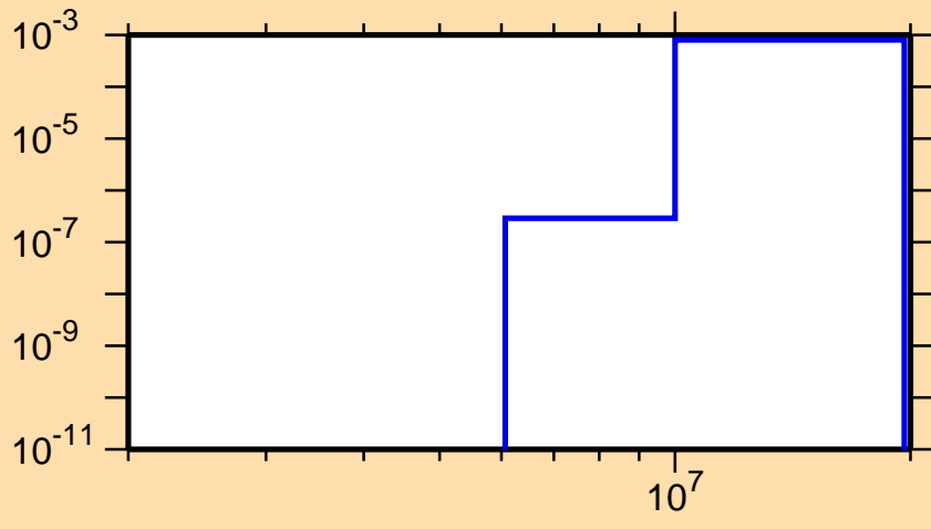
\sigma vs. E for ^{187}\text{Ta}(n,p)
