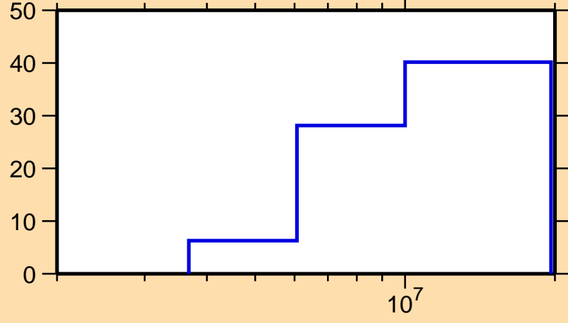
\Delta\sigma/\sigma vs. E for ^{187}\text{Ta}(n,ncont.)
