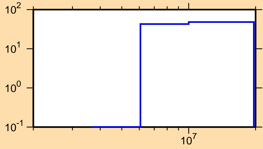
\Delta\sigma/\sigma vs. E for ^{187}\text{Ta}(n,p)
