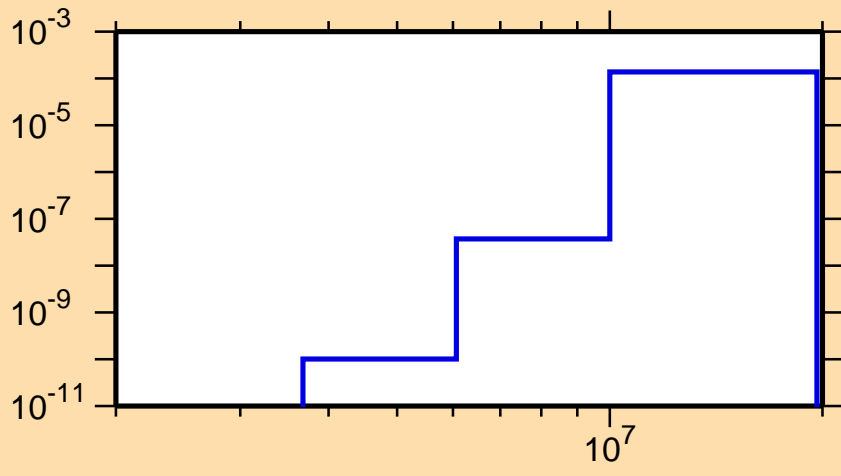
\sigma vs. E for ^{187}\text{Ta}(n,\alpha)
