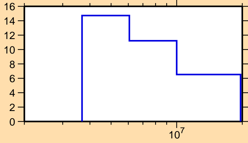
\Delta\sigma/\sigma vs. E for ^{187}\text{Ta}(n,el.)
