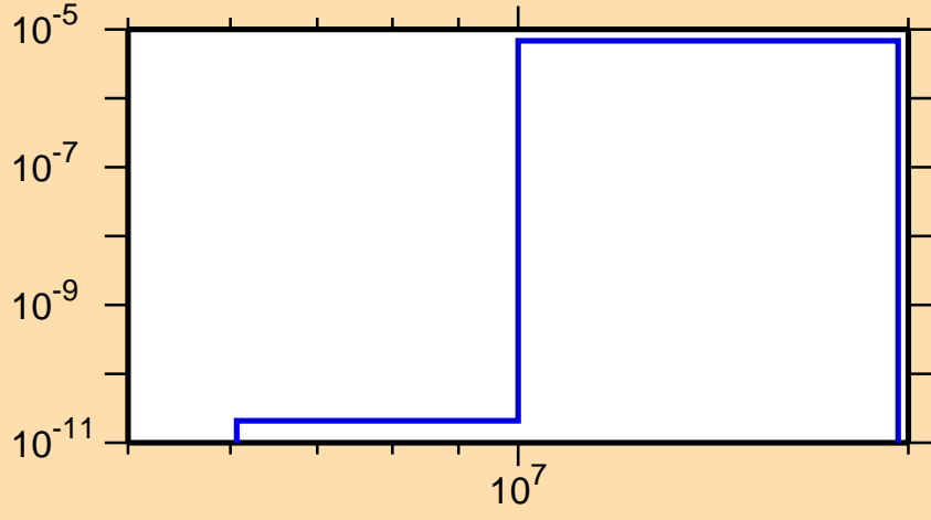
\sigma vs. E for ^{187}\text{Ta}(n,n\alpha)
