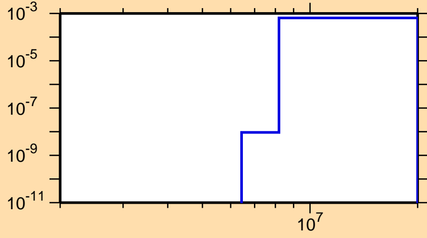
\sigma vs. E for ^{187}\text{Ta}(n,p)
