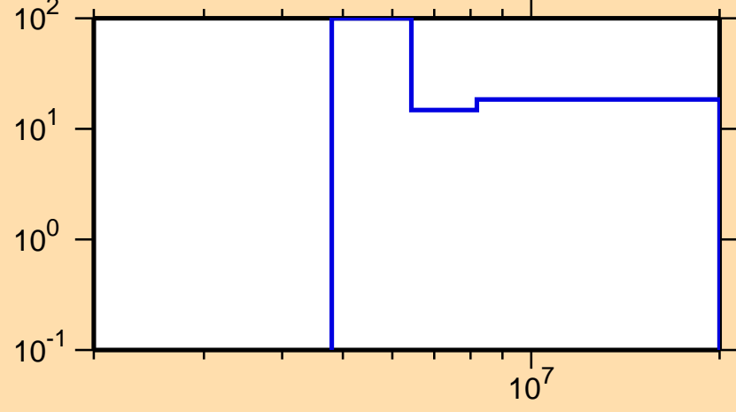
\Delta\sigma/\sigma vs. E for ^{187}\text{Ta}(n,2n)
