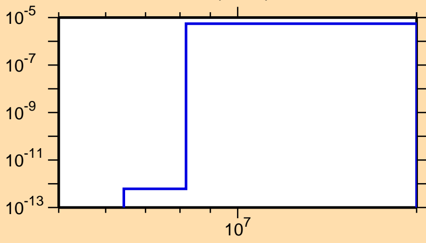
\sigma vs. E for ^{187}\text{Ta}(n,n\alpha)
