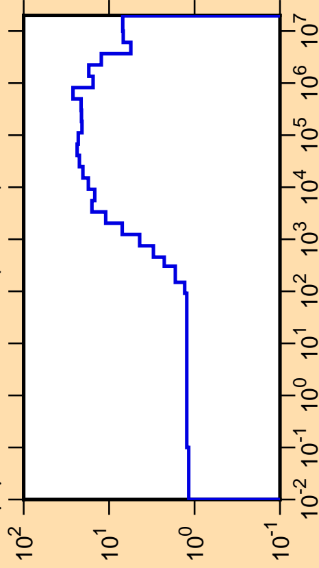
\Delta\mu/\mu vs. E for ^{188}\text{Ta}(\text{mt251})
