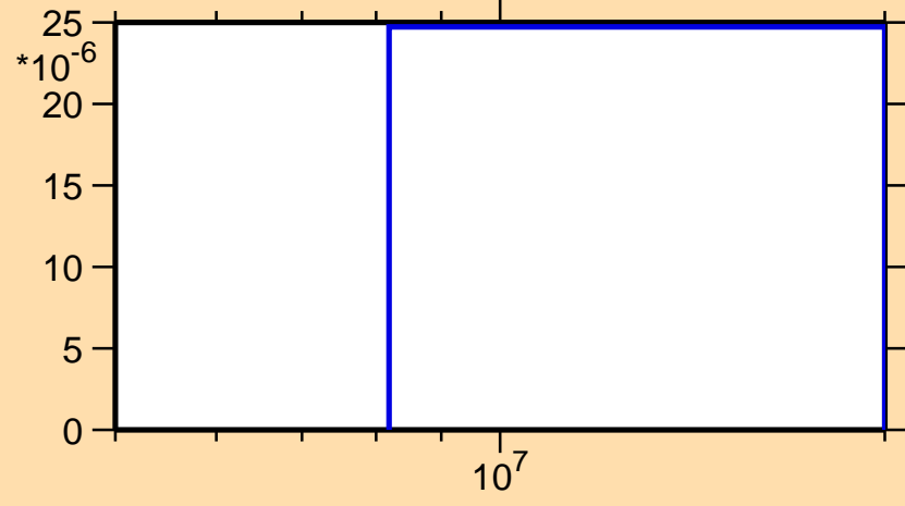
\sigma vs. E for ^{188}\text{Ta}(n,np)
