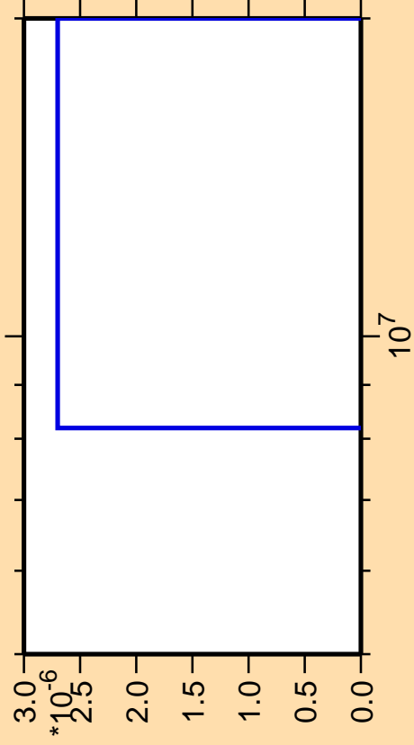
\Delta\sigma/\sigma vs. E for ^{188}\text{Ta}(\text{mt } 42)
