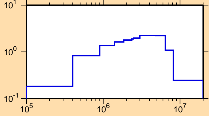
\sigma vs. E for ^{188}\text{Ta}(n,\text{inel.})
