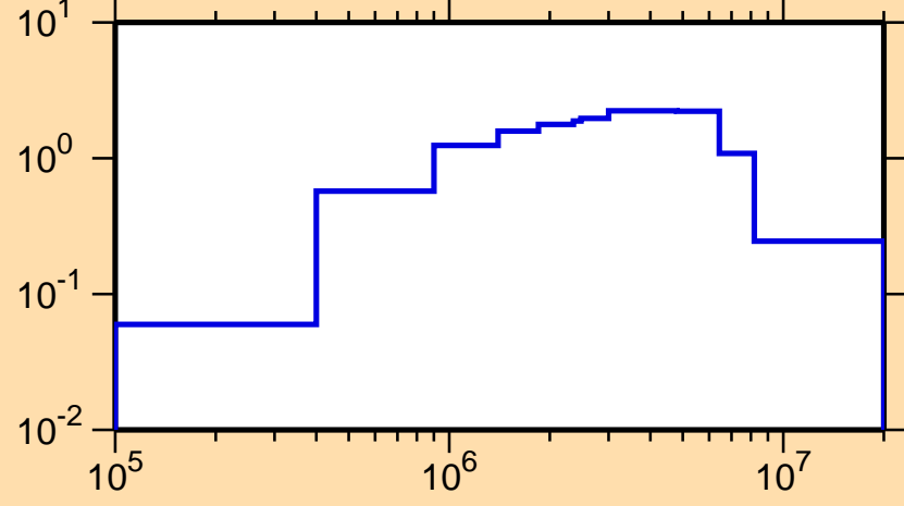
\sigma vs. E for ^{188}\text{Ta}(n,n_{\text{cont}}) .
