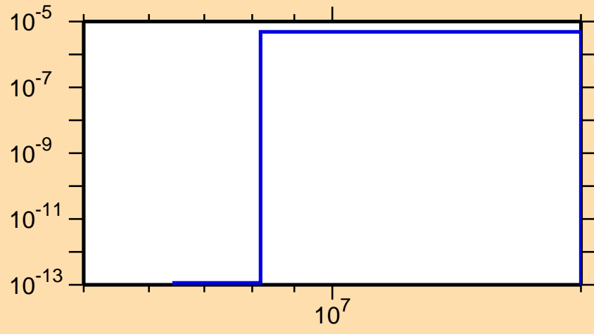
\sigma vs. E for ^{188}\text{Ta}(n,n\alpha)
