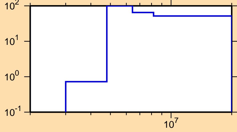
\Delta\sigma/\sigma vs. E for ^{188}\text{Ta}(n,p)
