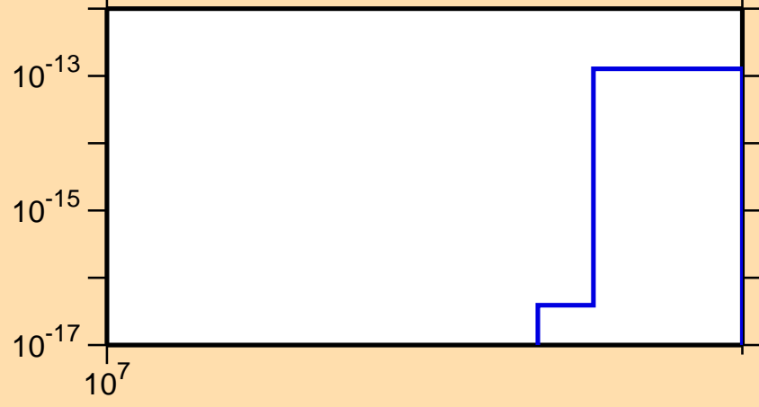
\sigma vs. E for ^{189}\text{Ta}(n,3n\alpha)
