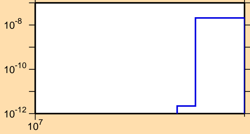
\sigma vs. E for ^{189}\text{Ta}(n,2np)
