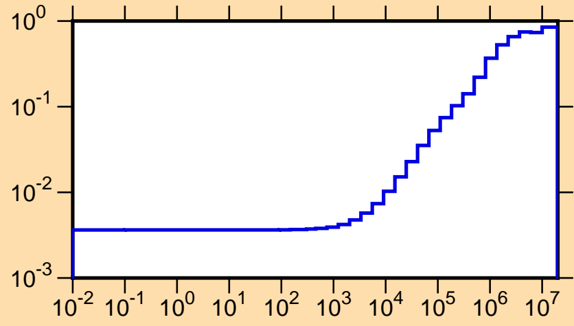
\mu vs. E for ^{189}\text{Ta}(\text{mt251})
