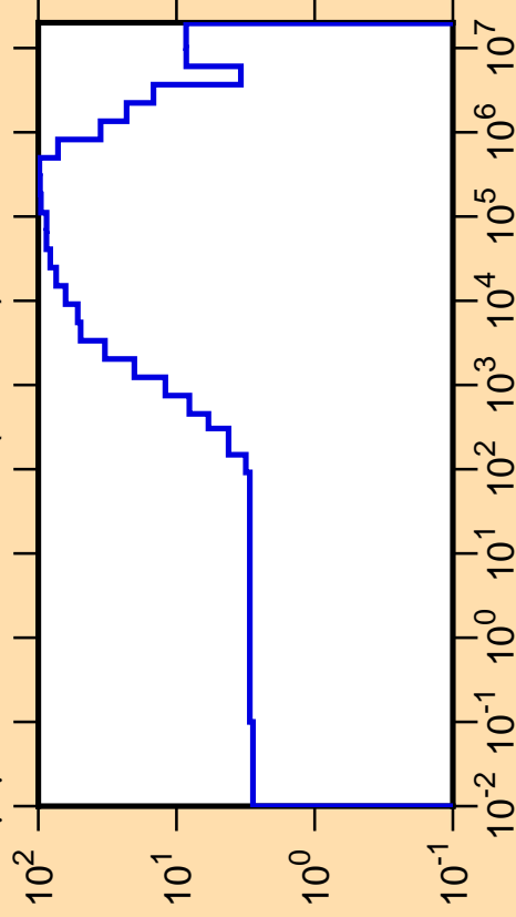
\Delta\mu/\mu vs. E for ^{189}\text{Ta}(\text{mt251})
