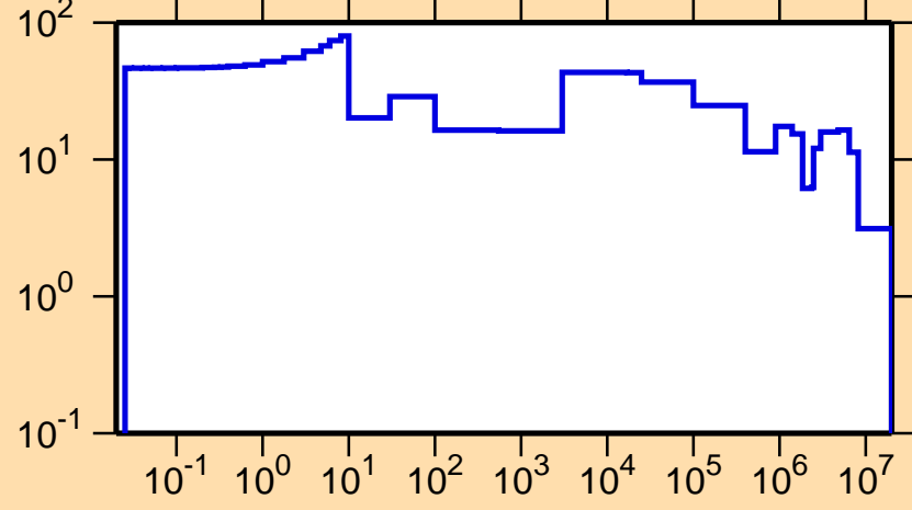
\Delta\sigma/\sigma vs. E for ^{189}\text{Ta}(n,\text{tot.})
