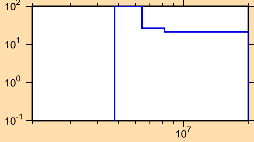
\Delta\sigma/\sigma vs. E for ^{189}\text{Ta}(n,2n)
