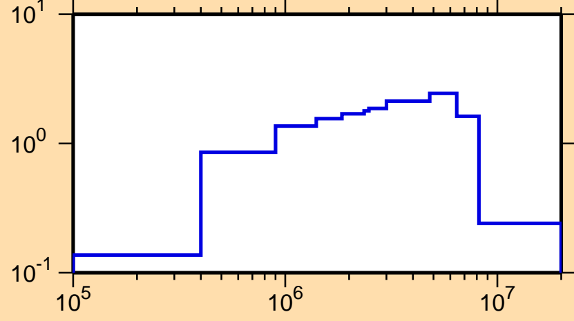
\sigma vs. E for ^{189}\text{Ta}(n,n\text{cont.})
