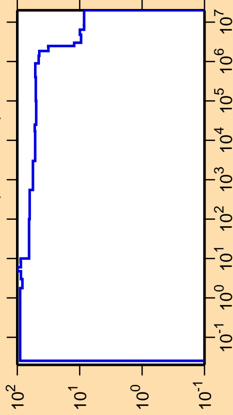
\Delta\sigma/\sigma vs. E for ^{189}\text{Ta}(n,\text{nonel.})
