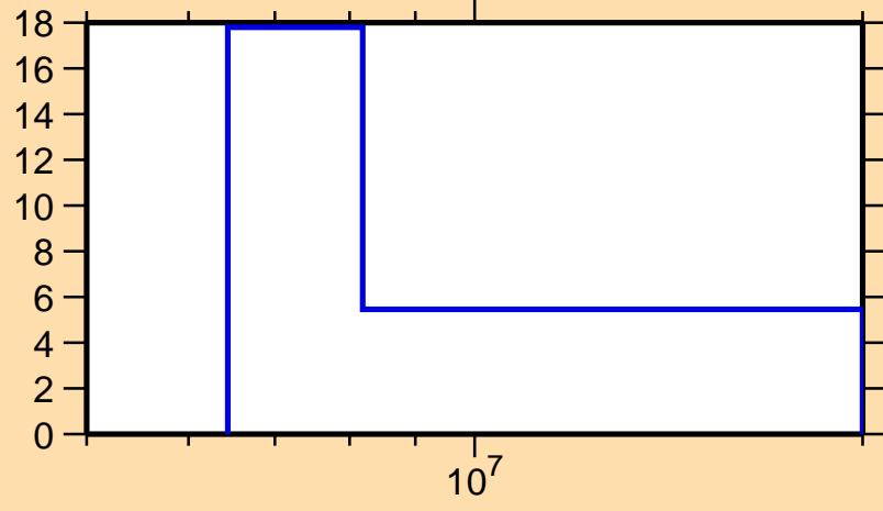
\Delta\sigma/\sigma vs. E for ^{189}\text{Ta}(n,el.)
