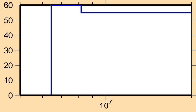
\Delta\sigma/\sigma vs. E for ^{189}\text{Ta}(n,ncont.)
