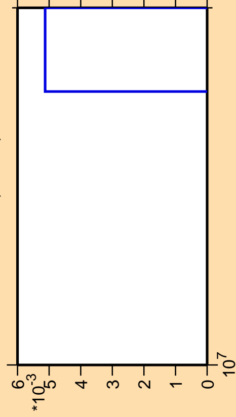
\Delta\sigma/\sigma vs. E for ^{190}\text{Ta} (mt 42)
