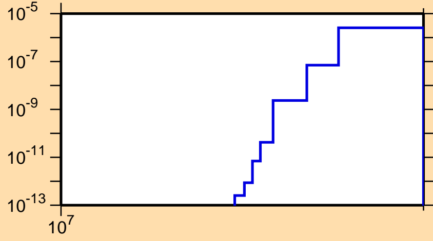
\sigma vs. E for ^{190}\text{Ta}(n,nt)
