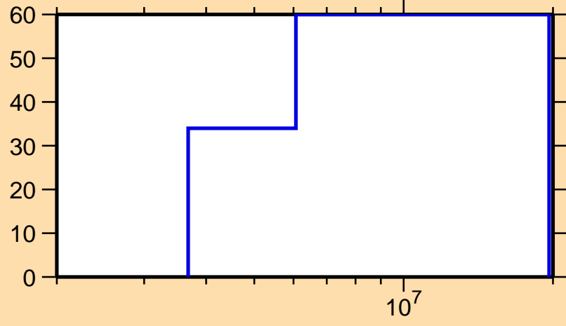
\Delta\sigma/\sigma vs. E for ^{190}\text{Ta}(n,ncont.)
