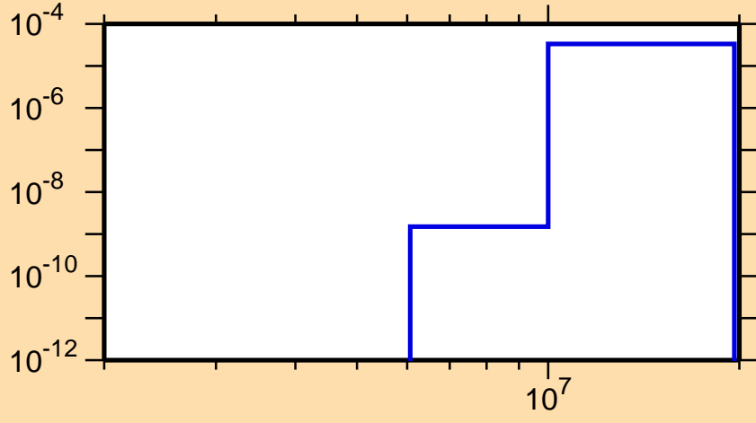
\sigma vs. E for ^{190}\text{Ta}(n,\alpha)
