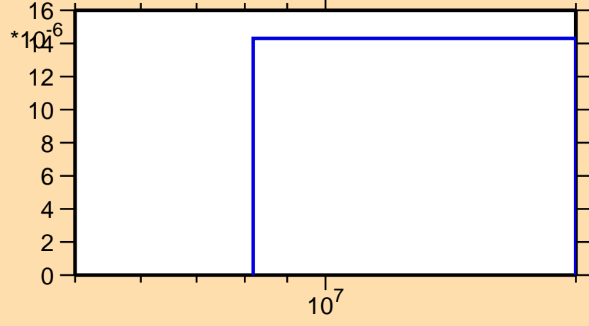
\sigma vs. E for ^{190}\text{Ta}(n,t)
