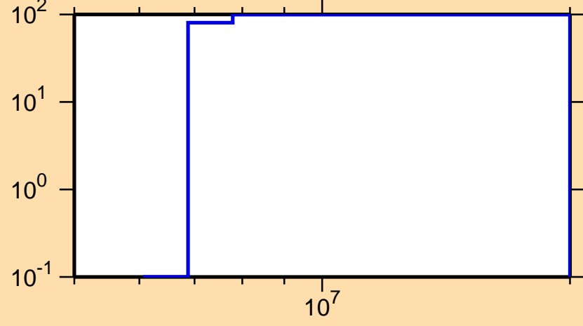
\Delta\sigma/\sigma vs. E for ^{191}\text{Ta}(n,p)
