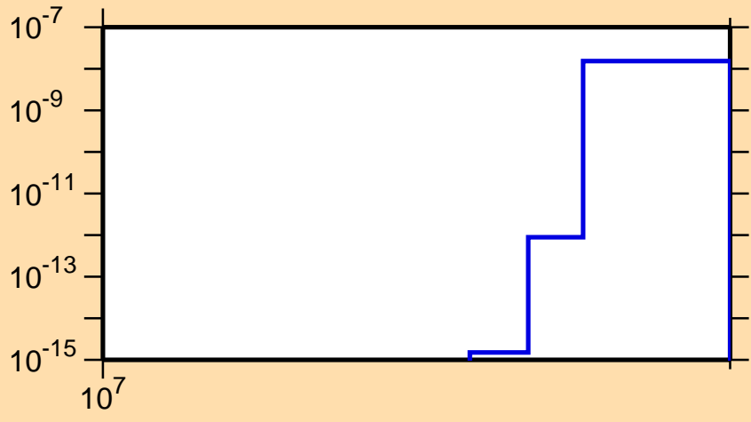
\sigma vs. E for ^{191}\text{Ta}(n,2np)
