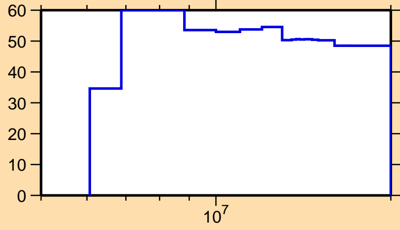
\Delta\sigma/\sigma vs. E for ^{191}\text{Ta}(n,ncont.)
