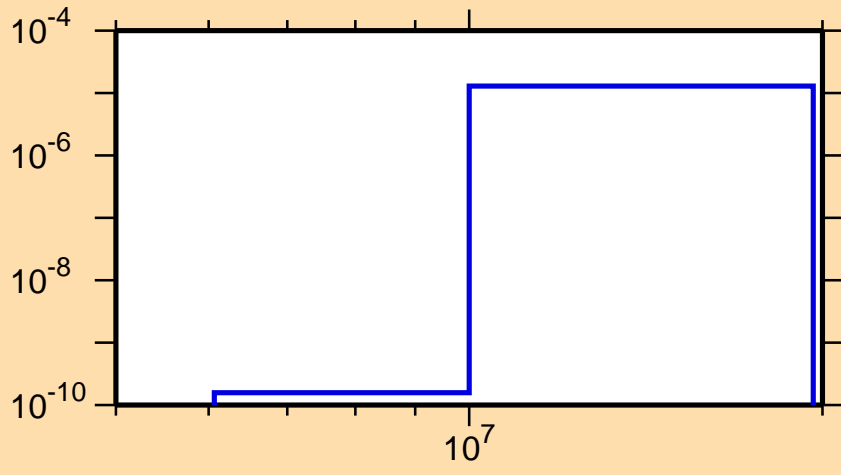
\sigma vs. E for ^{191}\text{Ta}(n,\alpha)
