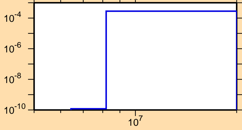
\sigma vs. E for ^{191}\text{Ta}(n,p)
