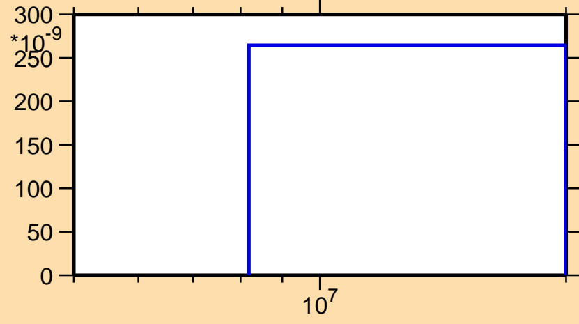
\sigma vs. E for ^{191}\text{Ta}(n,n\alpha)
