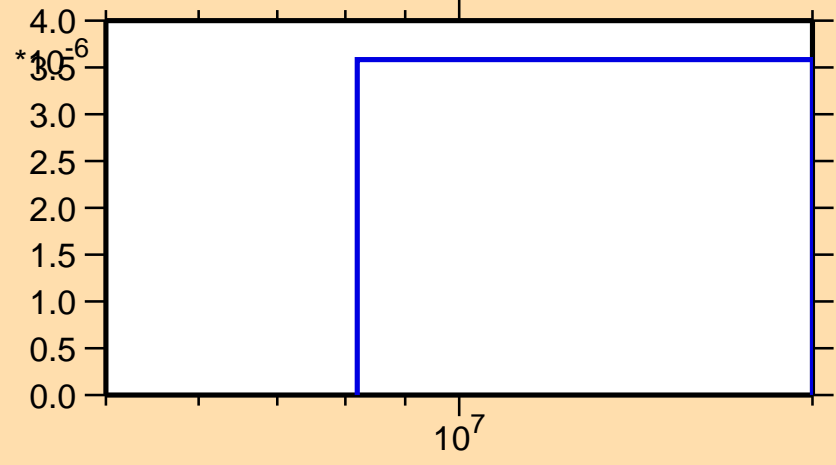
\sigma vs. E for ^{191}\text{Ta}(n,t)
