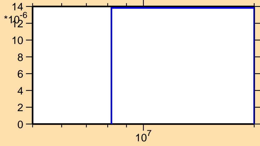
\sigma vs. E for ^{191}\text{Ta}(n,d)
