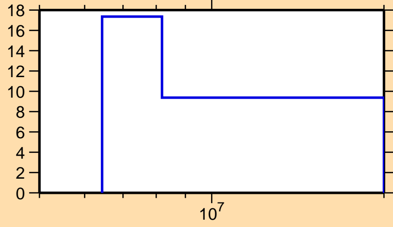
\Delta\sigma/\sigma vs. E for ^{191}\text{Ta}(n,el.)
