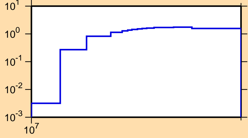
\sigma vs. E for ^{192}\text{Ta}(n,3n)
