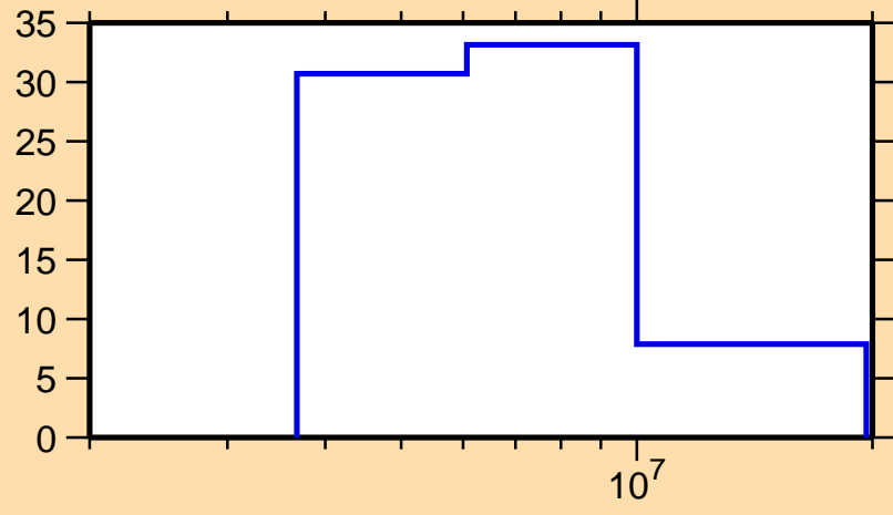
\Delta\sigma/\sigma vs. E for ^{192}\text{Ta}(n,el.)
