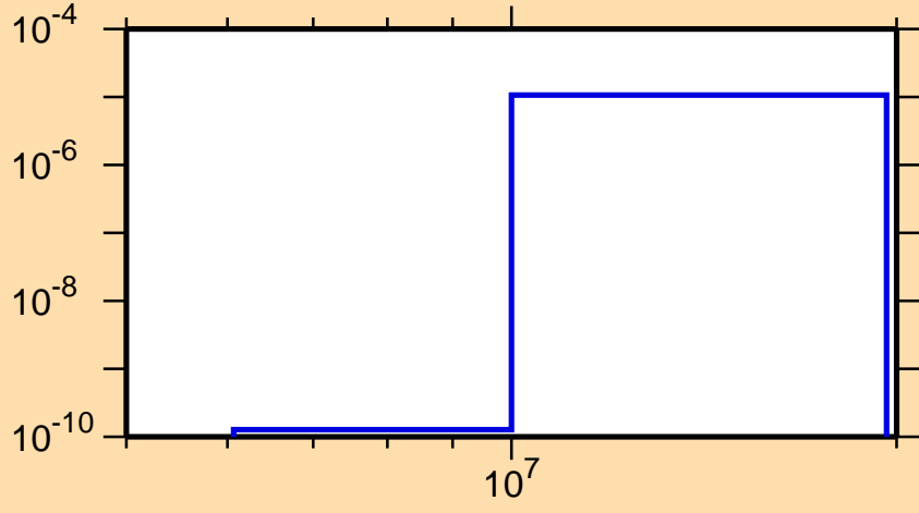
\sigma vs. E for ^{192}\text{Ta}(n,\alpha)
