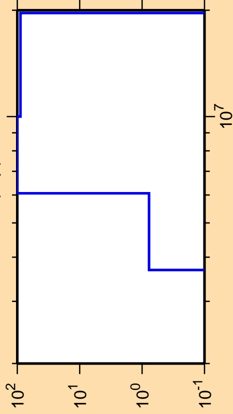
\Delta\sigma/\sigma vs. E for ^{192}\text{Ta}(n,p)
