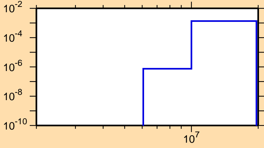
\sigma vs. E for ^{192}\text{Ta}(n,p)
