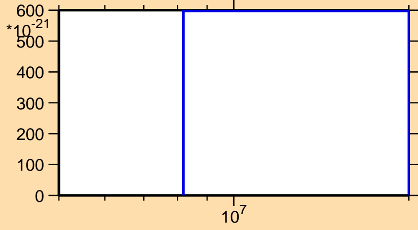
\sigma vs. E for ^{192}\text{Ta}(\text{mt } 42)
