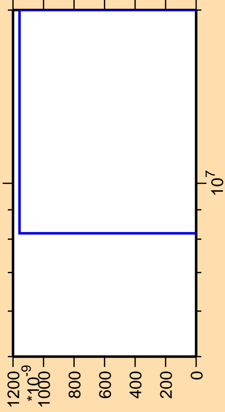
\Delta\sigma/\sigma vs. E for ^{192}\text{Ta}(\text{mt } 42)
