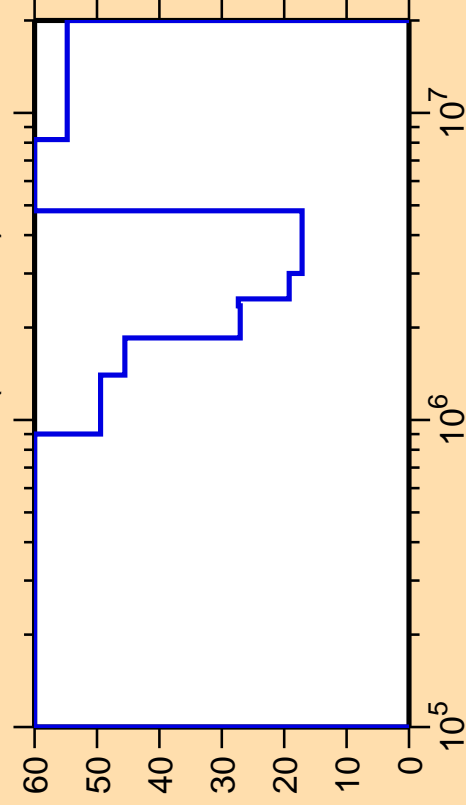
\Delta\sigma/\sigma vs. E for ^{192}\text{Ta}(n,n_{\text{cont}}) .
