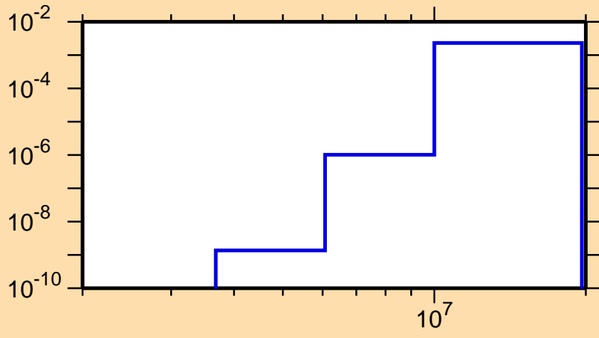
\sigma vs. E for ^{87}\text{Tc}(n,\text{He3})
