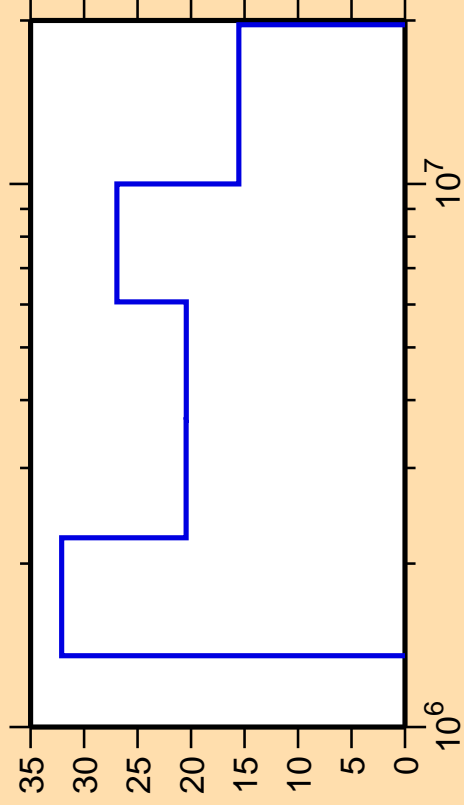
\Delta\sigma/\sigma vs. E for ^{87}\text{Tc}(n,n_2)
