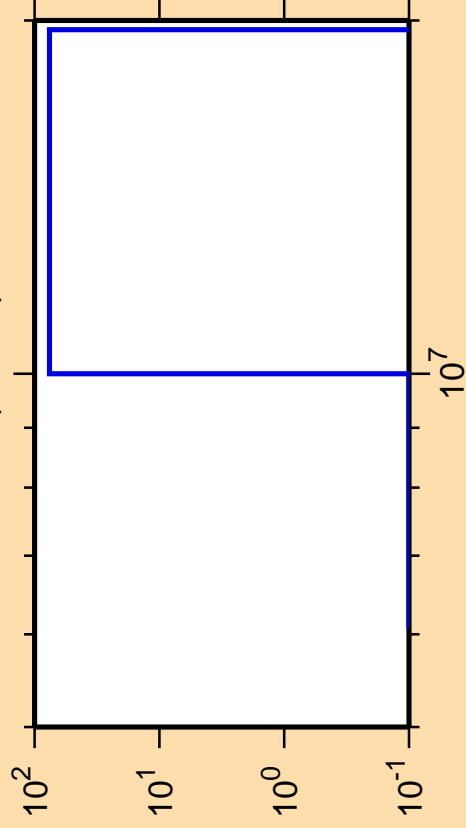
\Delta\sigma/\sigma vs. E for ^{87}\text{Tc} (mt 45)
