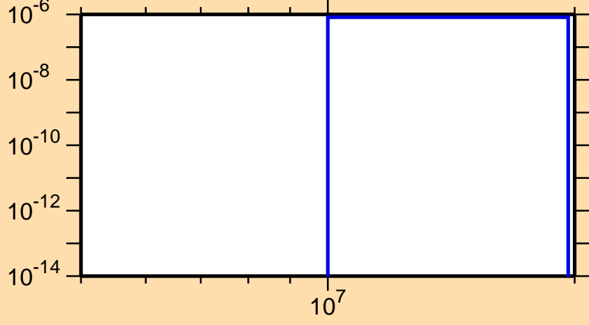
\sigma vs. E for ^{87}\text{Tc} (mt 45)
