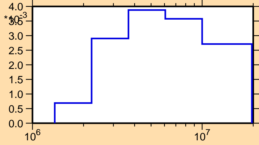
\sigma vs. E for ^{87}\text{Tc}(n,n_2)
