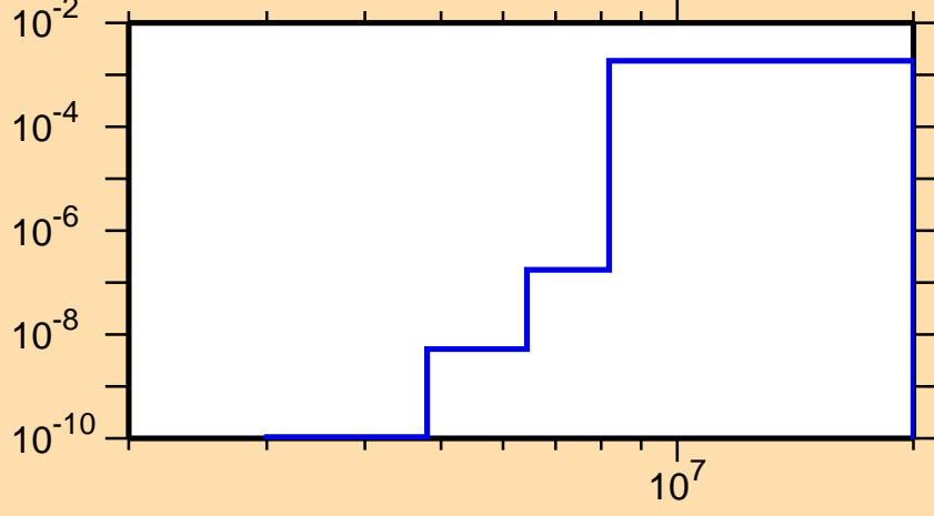
\sigma vs. E for ^{87}\text{Tc}(n,\text{He3})
