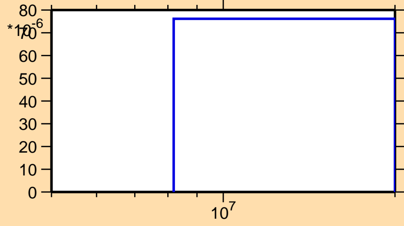
\sigma vs. E for ^{87}\text{Tc}(n,t)
