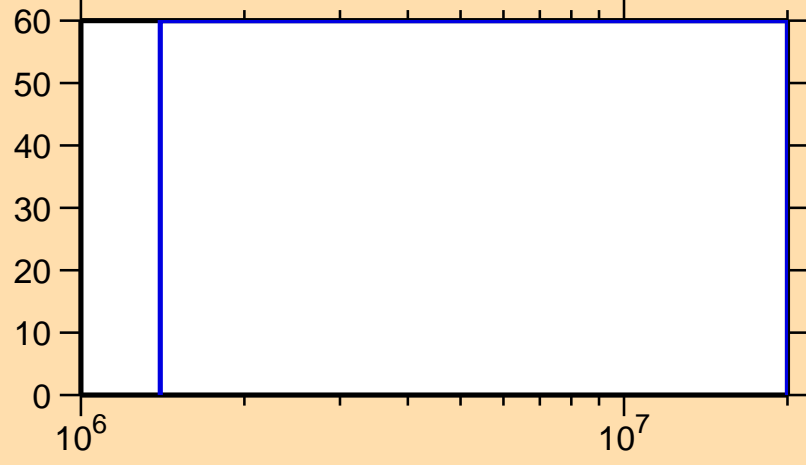
\Delta\sigma/\sigma vs. E for ^{87}\text{Tc}(n,ncont.)
