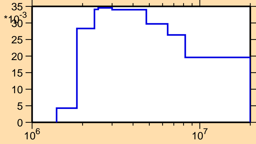
\sigma vs. E for ^{87}\text{Tc}(n,n_4)
