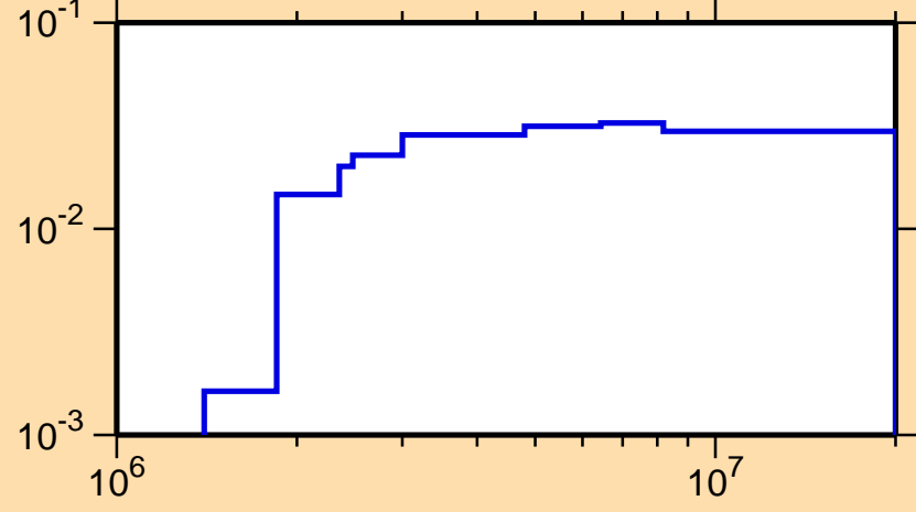
\sigma vs. E for ^{87}\text{Tc}(n,n\text{cont.})
