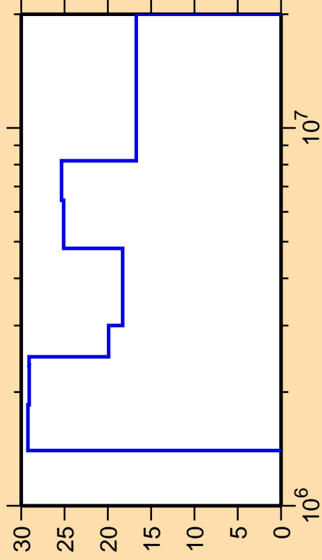
\Delta\sigma/\sigma vs. E for ^{87}\text{Tc}(n,n_4)
