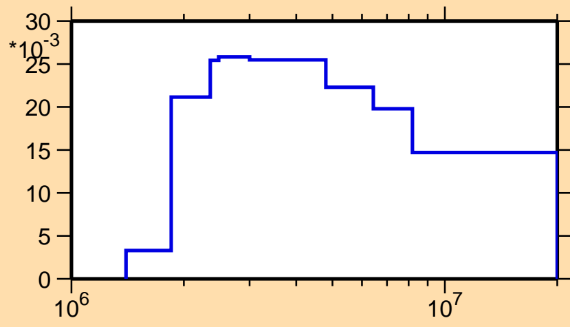
\sigma vs. E for ^{87}\text{Tc}(n,n_3)
