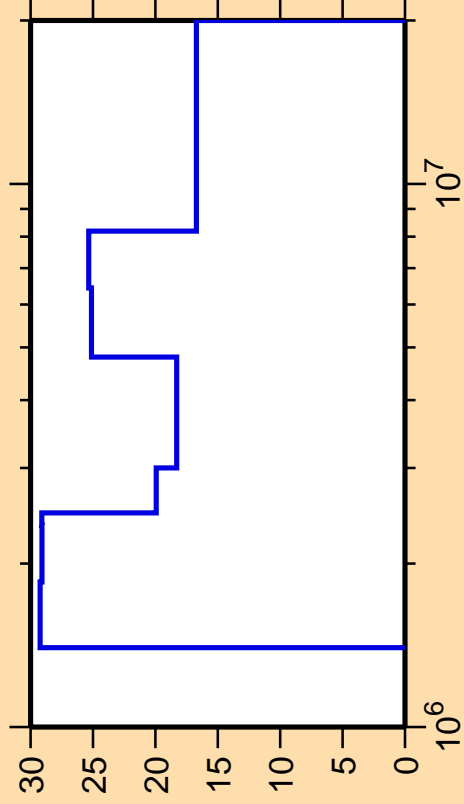
\Delta\sigma/\sigma vs. E for ^{87}\text{Tc}(n,n_3)
