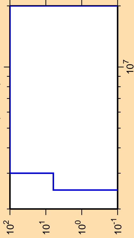
\Delta\sigma/\sigma vs. E for ^{87}\text{Tc}(n,\text{He3})
