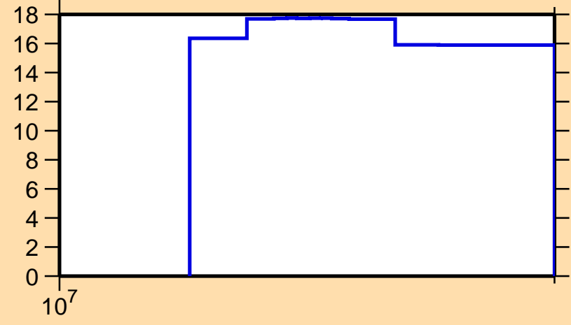
\Delta\sigma/\sigma vs. E for ^{88}\text{Tc}(n,\text{el.})
