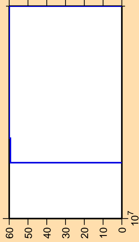
\Delta\sigma/\sigma vs. E for ^{88}\text{Tc}(n,n_1)
