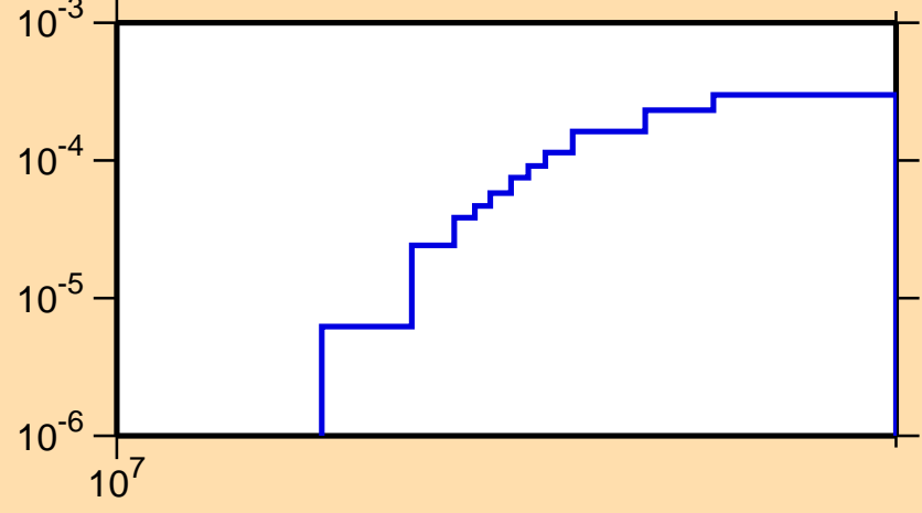
\sigma vs. E for ^{88}\text{Tc}(n,2n)
