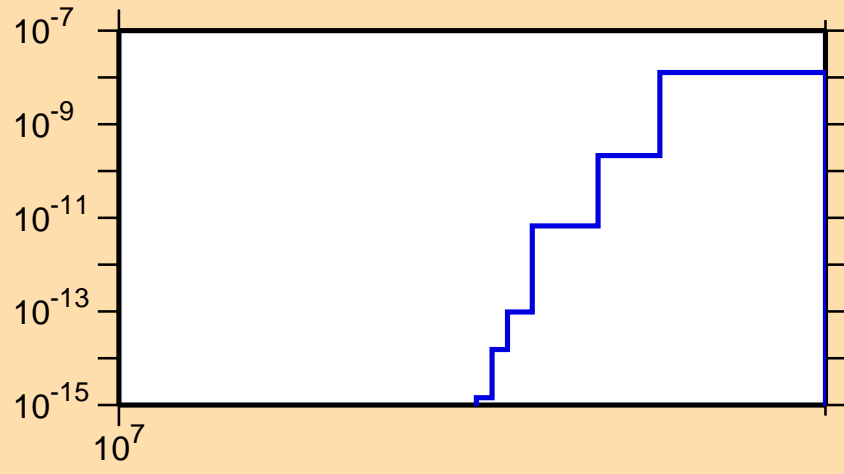
\sigma vs. E for ^{88}\text{Tc} (mt 34)
