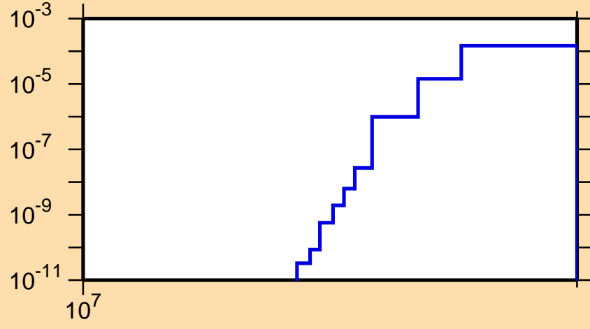
\sigma vs. E for ^{88}\text{Tc}(n,\text{pt})
