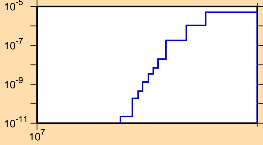
\sigma vs. E for ^{88}\text{Tc}(n,\text{nd})
