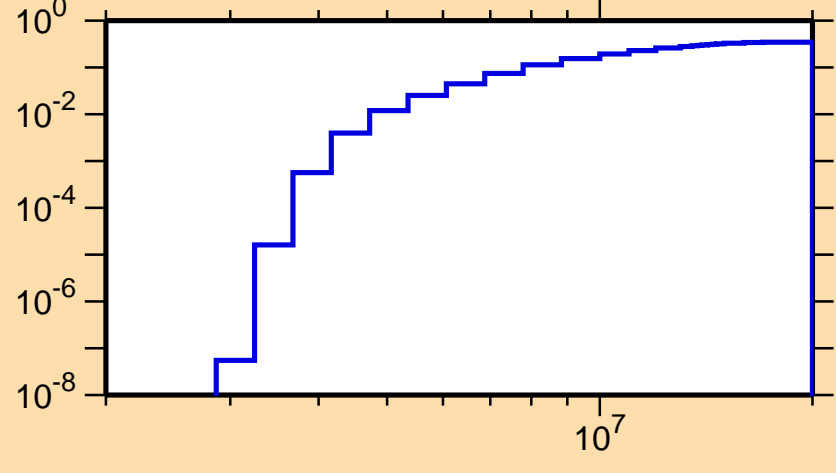
\sigma vs. E for ^{88}\text{Tc}(n,np)
