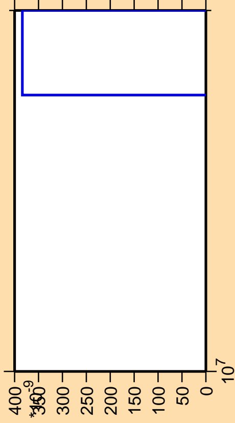
\Delta\sigma/\sigma vs. E for ^{88}\text{Tc}(n,nt)
