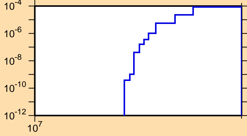
\sigma vs. E for ^{88}\text{Tc}(n,2np)
