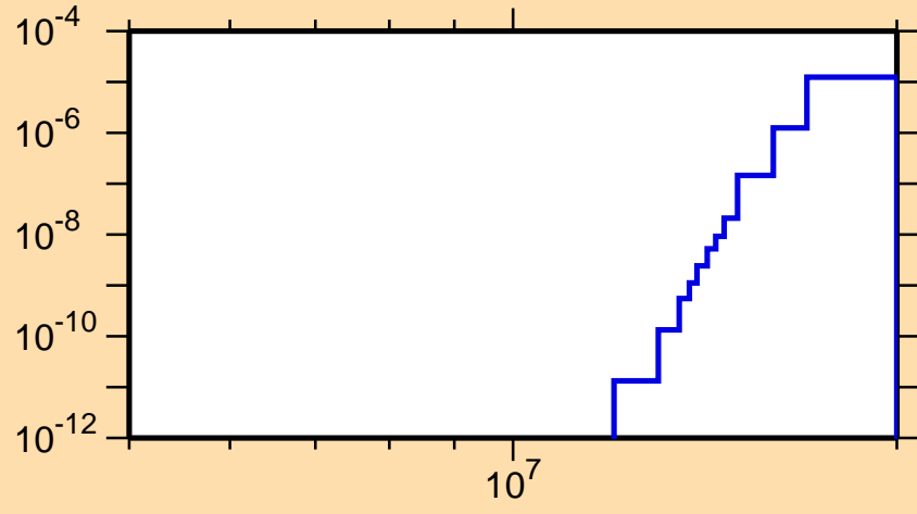
\sigma vs. E for ^{88}\text{Tc}(\text{mt } 45)
