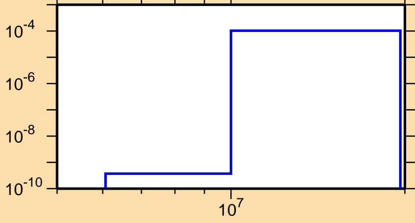
\sigma vs. E for ^{88}\text{Tc}(n,\alpha)
