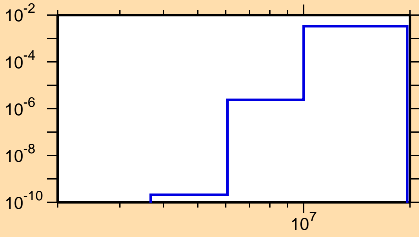
\sigma vs. E for ^{88}\text{Tc}(n,\text{He3})
