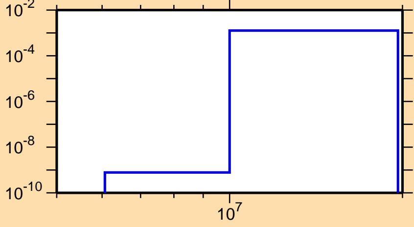
\sigma vs. E for ^{88}\text{Tc}(n,pd)
