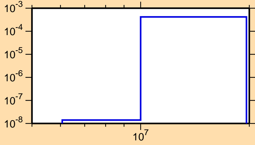
\sigma vs. E for ^{88}\text{Tc}(n,t)
