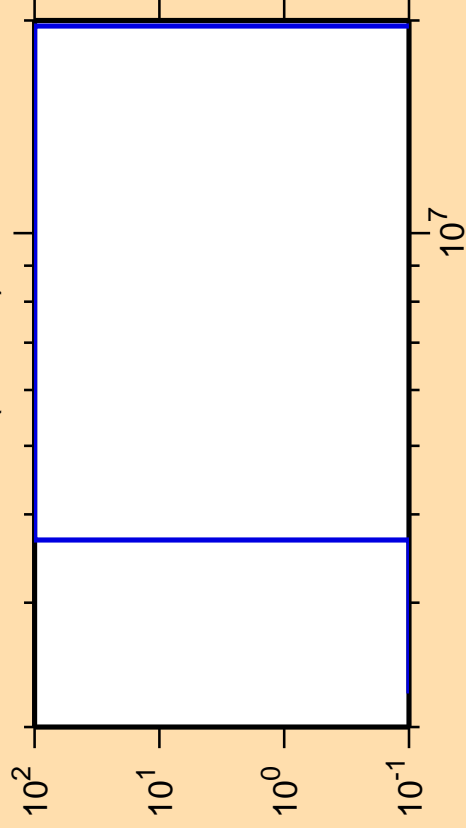
\Delta\sigma/\sigma vs. E for ^{88}\text{Tc}(n,\text{He3})
