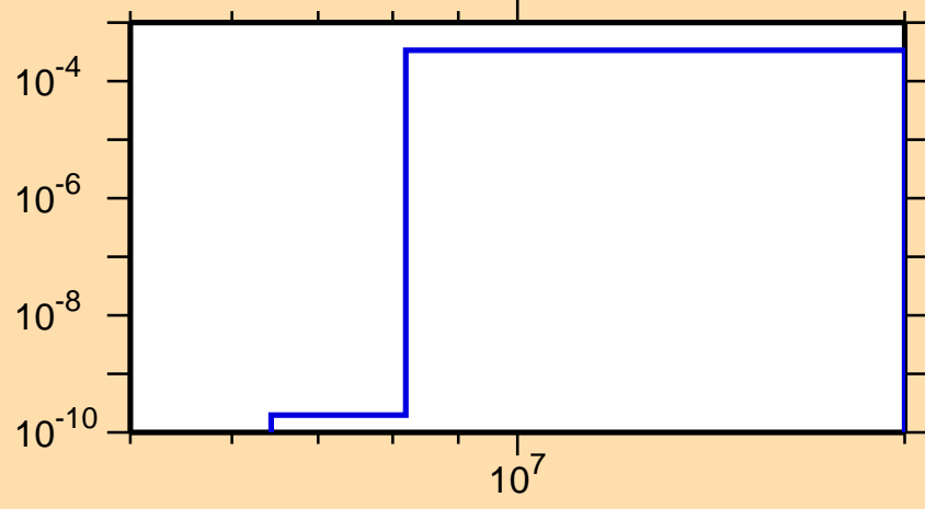
\sigma vs. E for ^{88}\text{Tc}(n,t)
