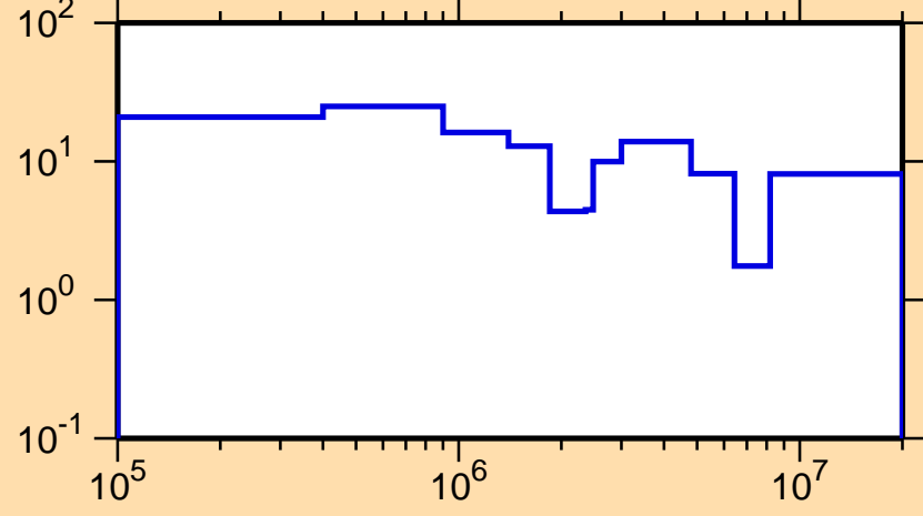
\Delta\sigma/\sigma vs. E for ^{88}\text{Tc}(n,\text{tot.})
