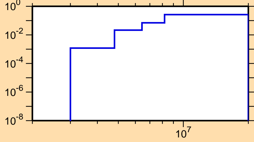
\sigma vs. E for ^{88}\text{Tc}(n,np)
