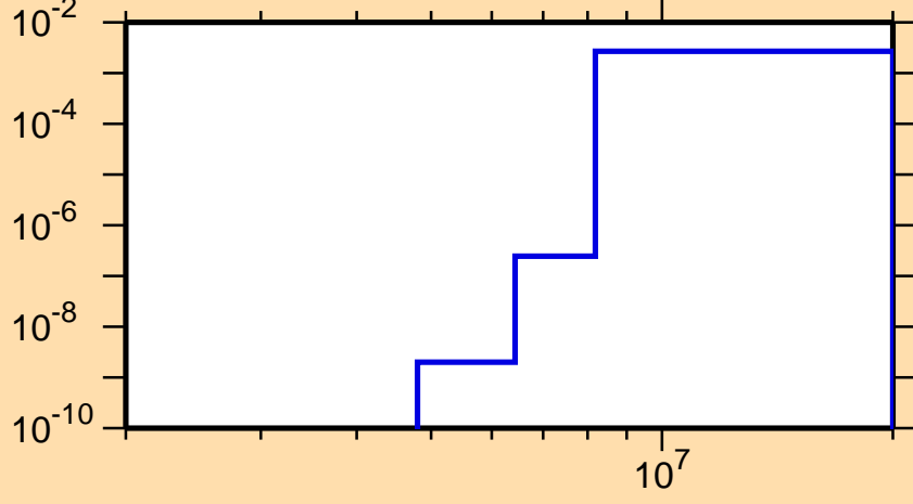
\sigma vs. E for ^{88}\text{Tc}(n,\text{He3})
