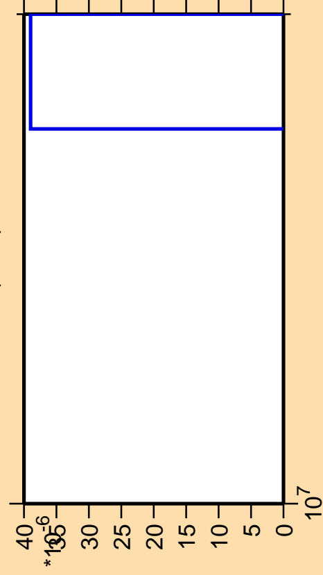
\Delta\sigma/\sigma vs. E for ^{88}\text{Tc}(n,nt)
