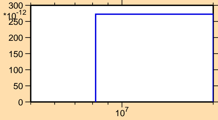
\sigma vs. E for ^{88}\text{Tc}(\text{mt } 34)
