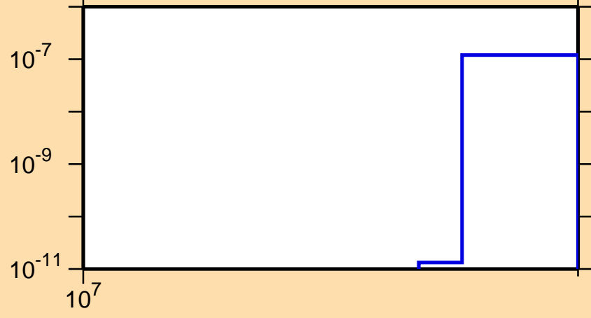
\sigma vs. E for ^{89}\text{Tc}(n,\text{pt})
