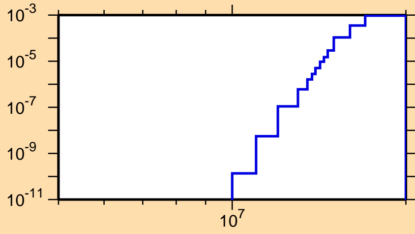
\sigma vs. E for ^{89}\text{Tc}(n,t)
