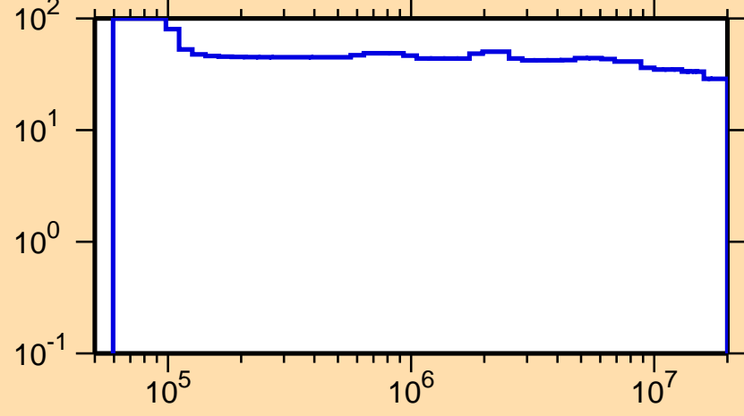
\Delta\sigma/\sigma vs. E for ^{89}\text{Tc}(n,n_1)
