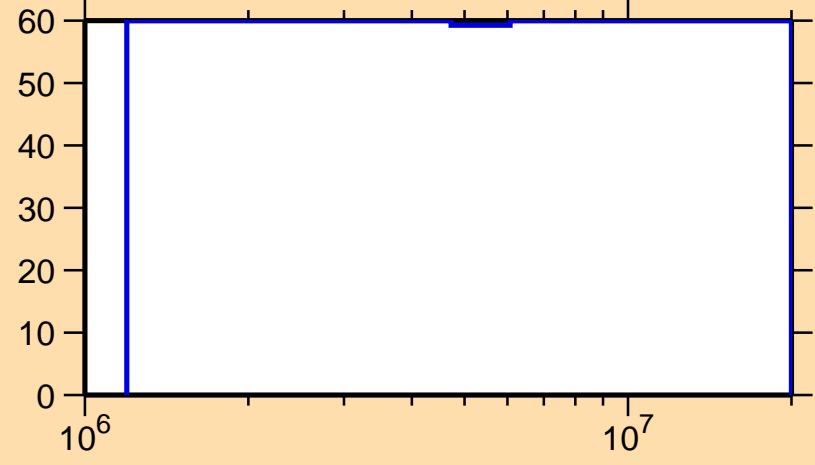
\Delta\sigma/\sigma vs. E for ^{89}\text{Tc}(n,ncont.)
