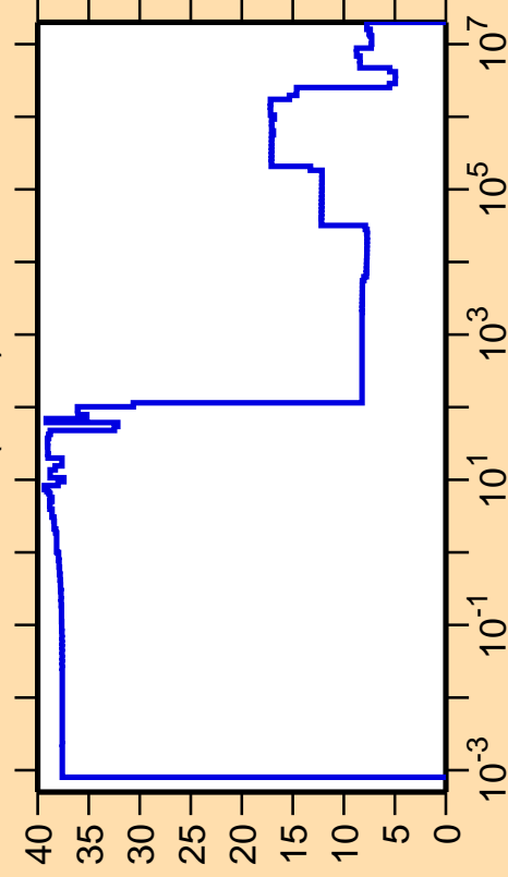
\Delta\sigma/\sigma vs. E for ^{89}\text{Tc}(n,\text{el.})
