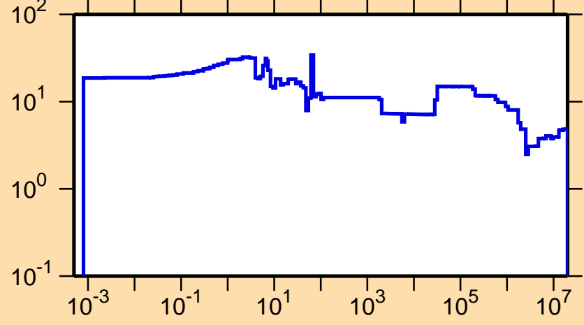
\Delta\sigma/\sigma vs. E for ^{89}\text{Tc}(n,\text{tot.})
