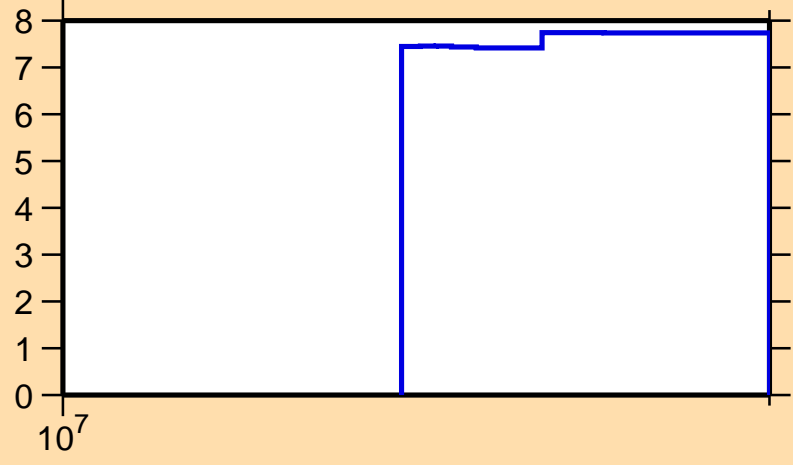
\Delta\sigma/\sigma vs. E for ^{89}\text{Tc}(n,\text{el.})
