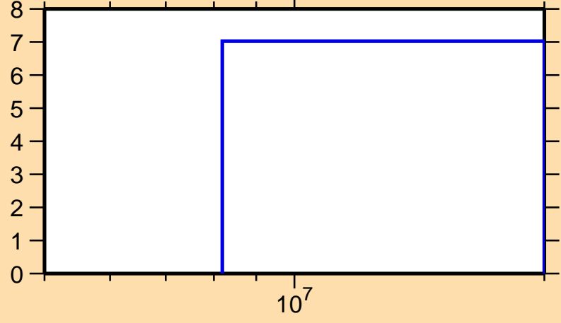
\Delta\sigma/\sigma vs. E for ^{89}\text{Tc}(n,\text{el.})
