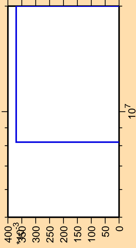
\Delta\sigma/\sigma vs. E for ^{89}\text{Tc} (mt 34)
