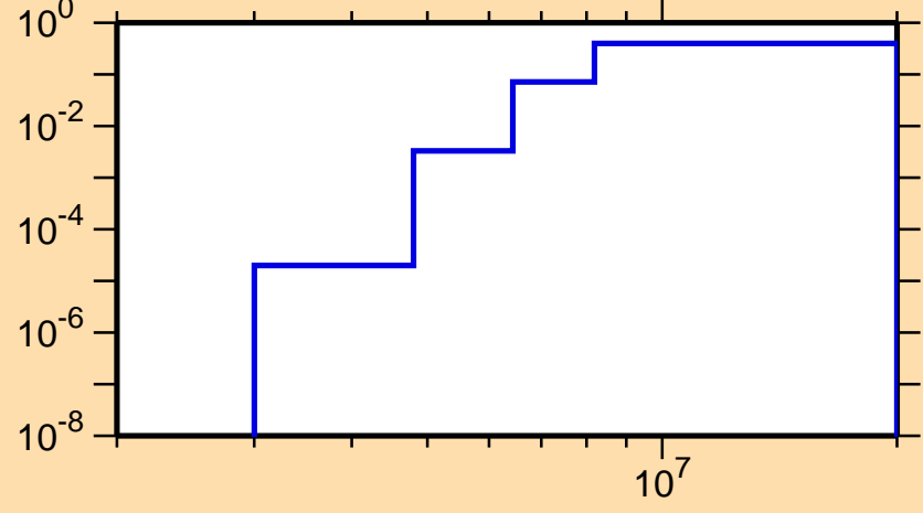
\sigma vs. E for ^{89}\text{Tc}(n,np)
