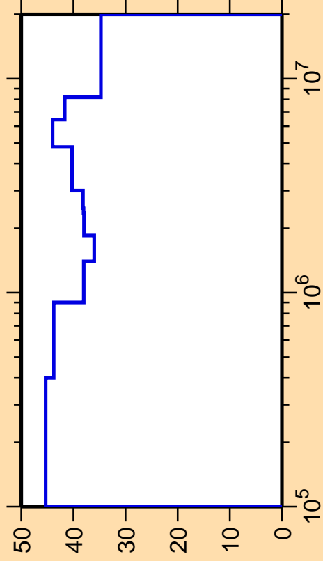
\Delta\sigma/\sigma vs. E for ^{89}\text{Tc}(n,n_2)
