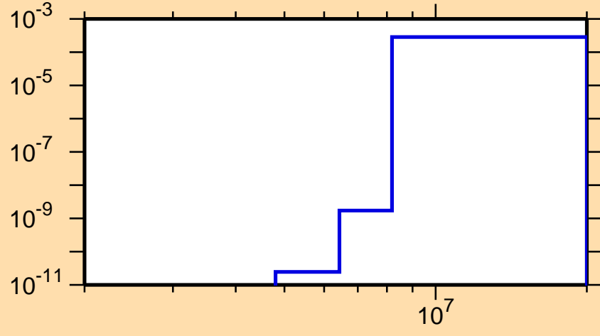
\sigma vs. E for ^{89}\text{Tc}(n,\text{He3})
