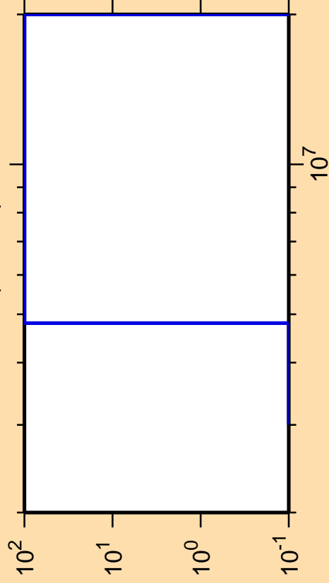
\Delta\sigma/\sigma vs. E for ^{89}\text{Tc}(n,\text{He3})
