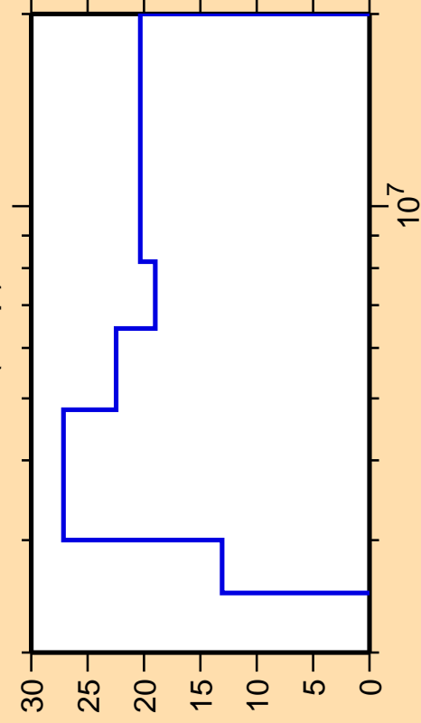
\Delta\sigma/\sigma vs. E for ^{89}\text{Tc}(n,np)
