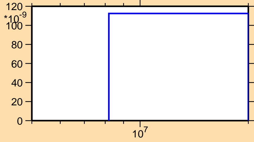
\sigma vs. E for ^{89}\text{Tc} (mt 45)
