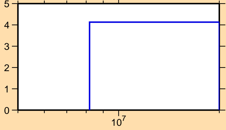
\Delta\sigma/\sigma vs. E for ^{89}\text{Tc}(n,\text{tot.})
