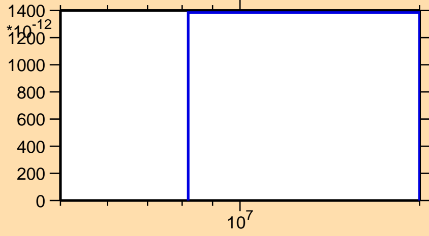
\sigma vs. E for ^{89}\text{Tc}(\text{mt117})
