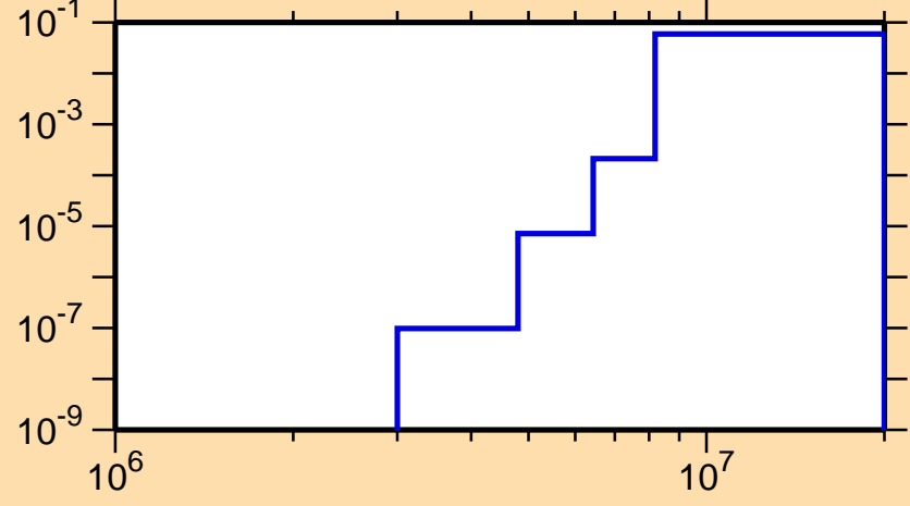
\sigma vs. E for ^{89}\text{Tc}(n,p\alpha)
