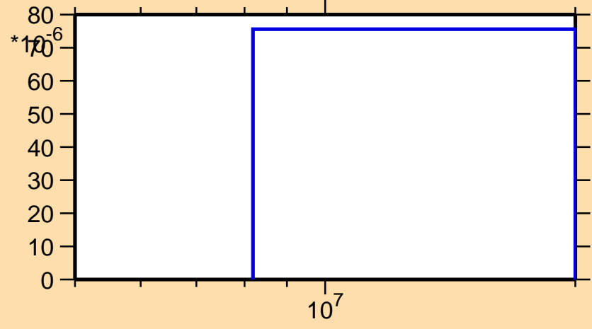
\sigma vs. E for ^{89}\text{Tc}(n,2n)
