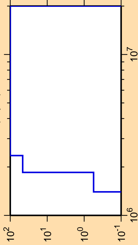
\Delta\sigma/\sigma vs. E for ^{89}\text{Tc}(n,p\alpha)
