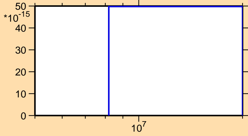
\sigma vs. E for ^{89}\text{Tc} (mt 34)
