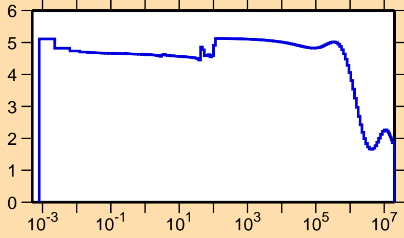
\sigma vs. E for ^{89}\text{Tc}(n,\text{el.})
