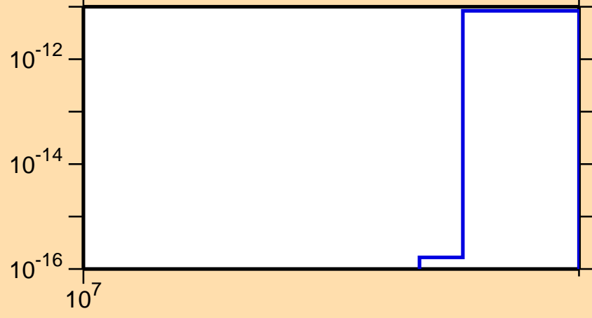
\sigma vs. E for ^{89}\text{Tc} (mt 34)
