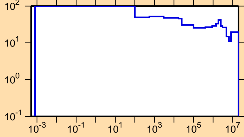
\Delta\sigma/\sigma vs. E for ^{89}\text{Tc}(n,\text{el.})
