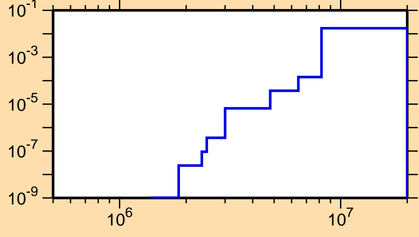
\sigma vs. E for ^{89}\text{Tc}(n,d)
