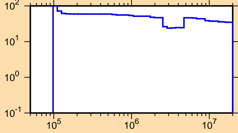
\Delta\sigma/\sigma vs. E for ^{90}\text{Tc}(n,n_1)
