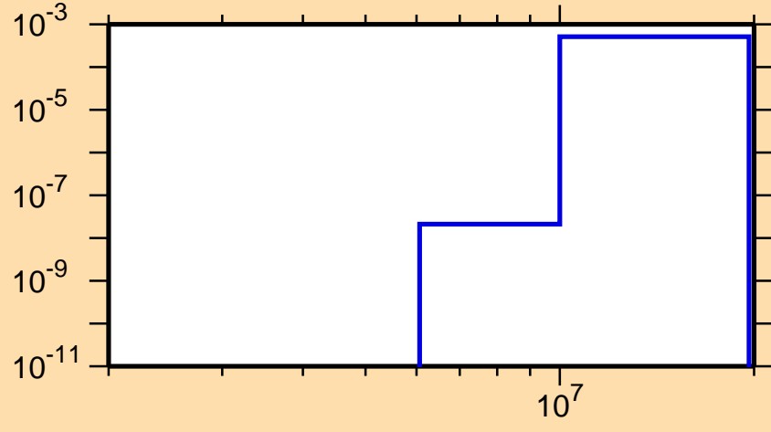
\sigma vs. E for ^{90}\text{Tc}(n,\text{He3})
