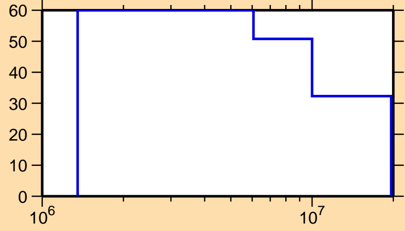
\Delta\sigma/\sigma vs. E for ^{90}\text{Tc}(n,ncont.)
