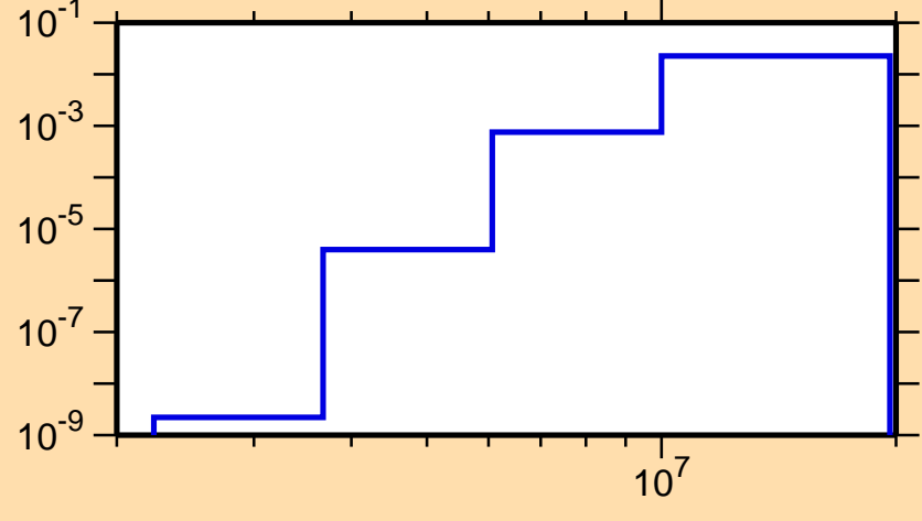
\sigma vs. E for ^{90}\text{Tc}(n,d)
