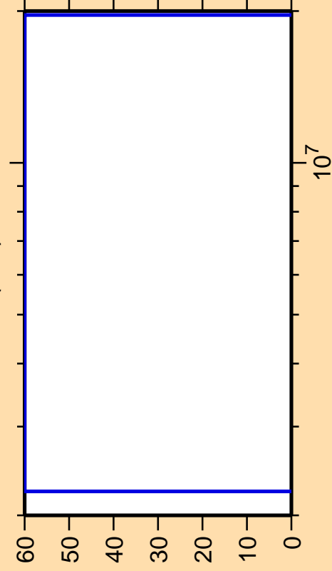
\Delta\sigma/\sigma vs. E for ^{90}\text{Tc}(n,d)
