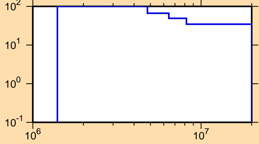
\Delta\sigma/\sigma vs. E for ^{90}\text{Tc}(n,ncont.)
