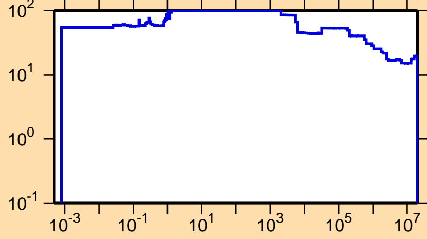
\Delta\sigma/\sigma vs. E for ^{90}\text{Tc}(n,\text{nonel.})
