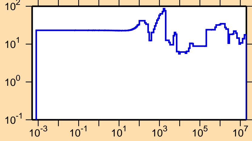
\Delta\sigma/\sigma vs. E for ^{90}\text{Tc}(n,\text{el.})
