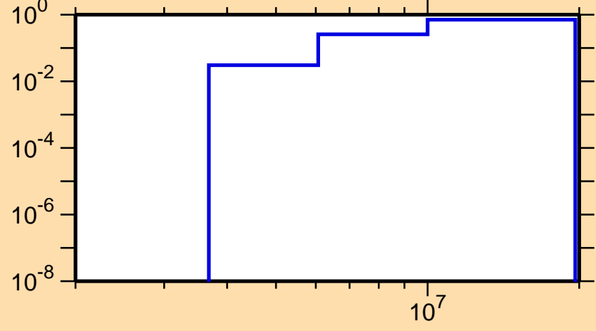
\sigma vs. E for ^{90}\text{Tc}(n,np)
