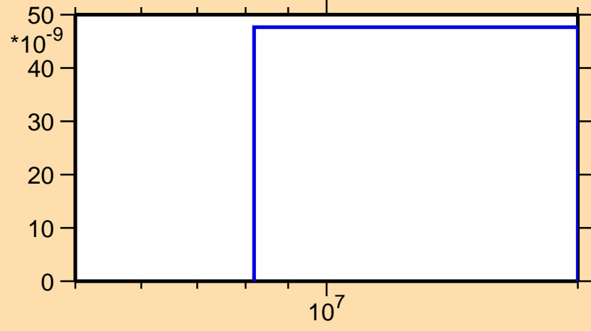
\sigma vs. E for ^{90}\text{Tc}(\text{mt } 45)
