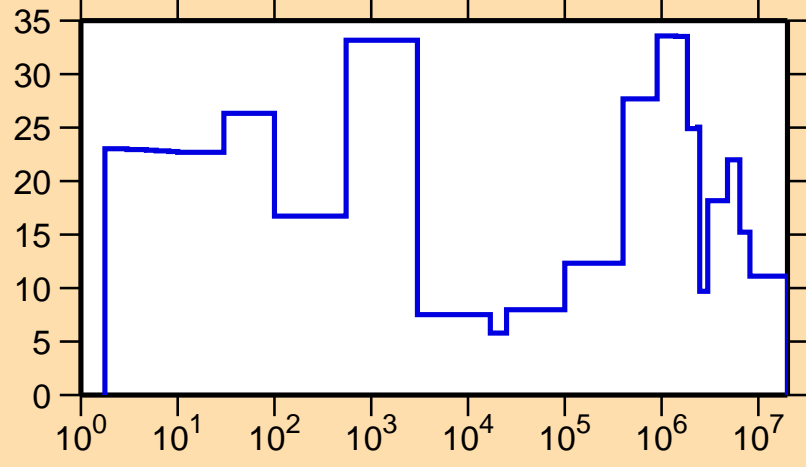
\Delta\sigma/\sigma vs. E for ^{90}\text{Tc}(n,el.)
