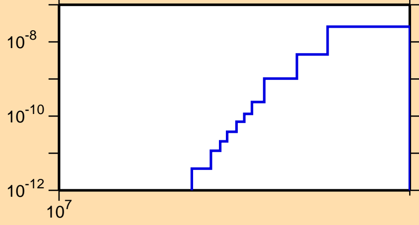
\sigma vs. E for ^{90}\text{Tc}(\text{mt117})
